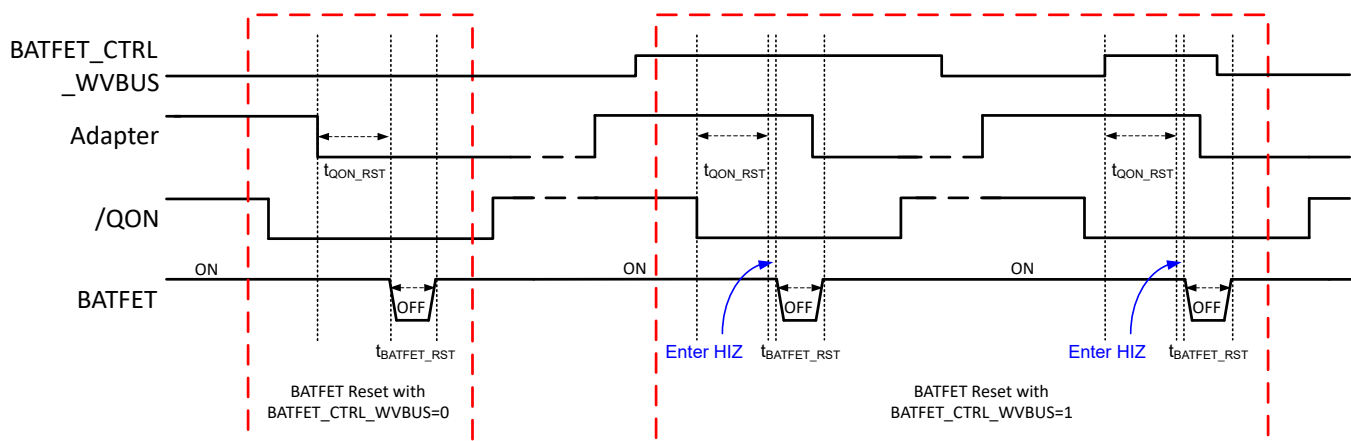
图 8-7. System Power Reset Timing
