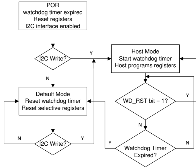
☒ 7-15. Watchdog Timer Flow Chart
