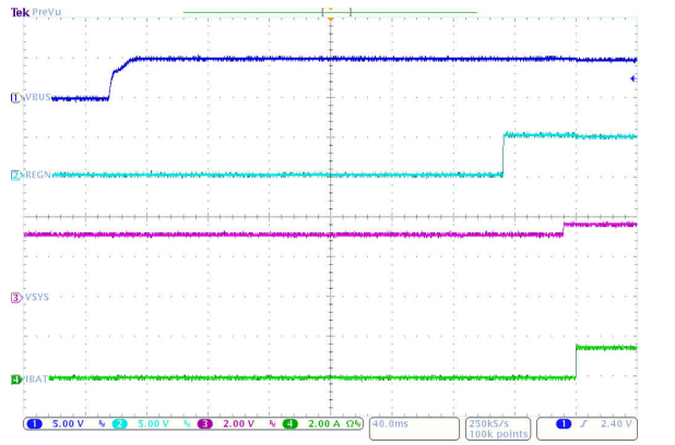
図 8-6. Power Up with Charge Enabled
