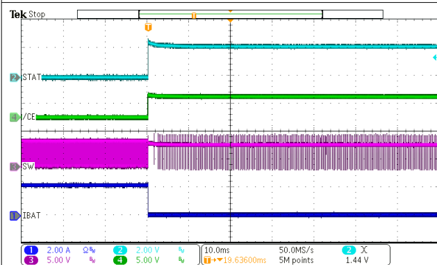
10-8. PWM Switching in Buck Mode
