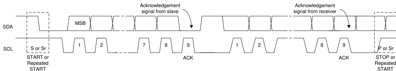
FIG 9-14. Data Transfer on the I²C Bus
