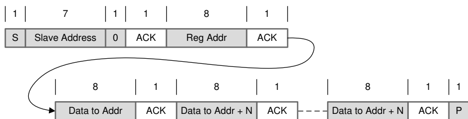
FIG 9-18. Multi-Write
