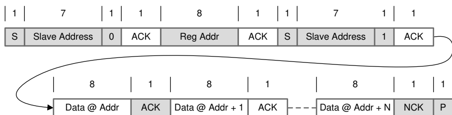
FIG 9-19. Multi-Read
