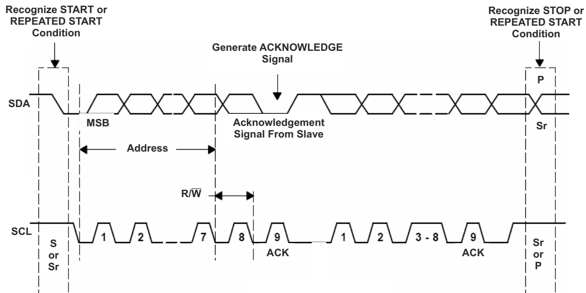
7-7. Bus Protocol
