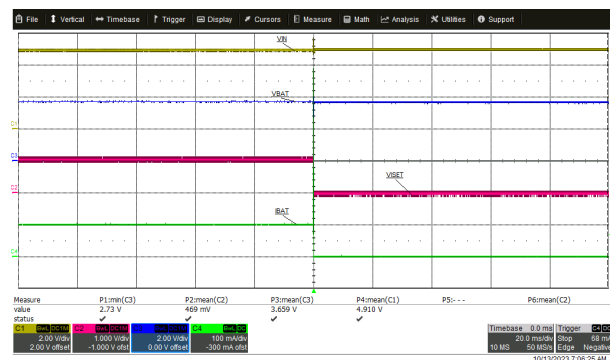
図 9-5. Wake up from Factory Mode with Adapter Insertion
