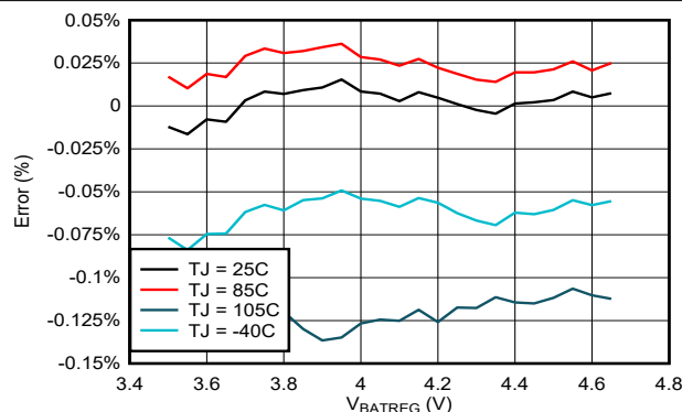
7-1. Battery Regulation Voltage Accuracy vs. VBATREG Setting
