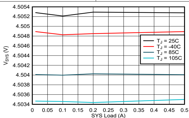
7-4. SYS Load Regulation
