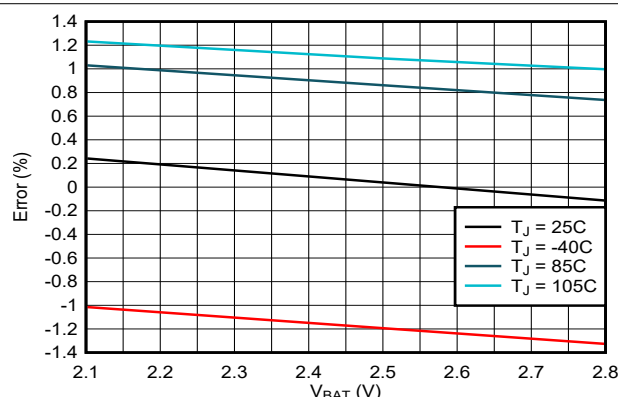
7-1. Battery Regulation Voltage Accuracy vs. VBATREG Setting
