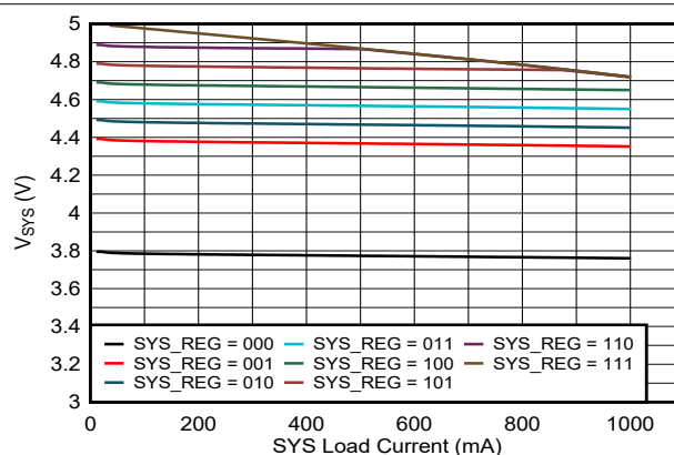
7-4. SYS Load Regulation
