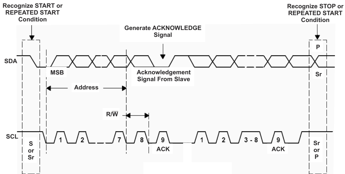
Figure 8-9. Bus Protocol
