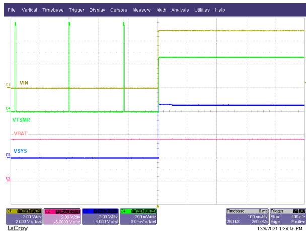
9-2. Power Up with IN Supply Insertion with No Battery
