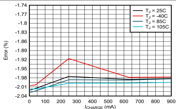
7-2. Charge Current Accuracy vs. ICHARGE Setting
