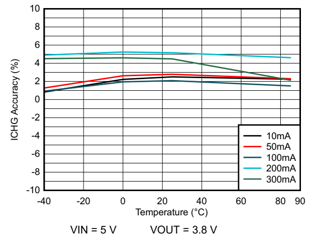
Figure 6-4. ICHG Accuracy vs. Temperature
