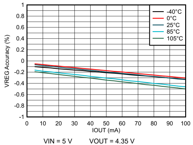
Figure 6-2. Load Regulation
