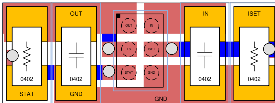
FIG 10-1. BQ25175 Board Layout Example
