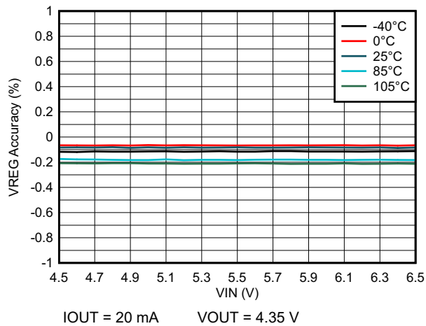
Figure 6-1. Line Regulation
