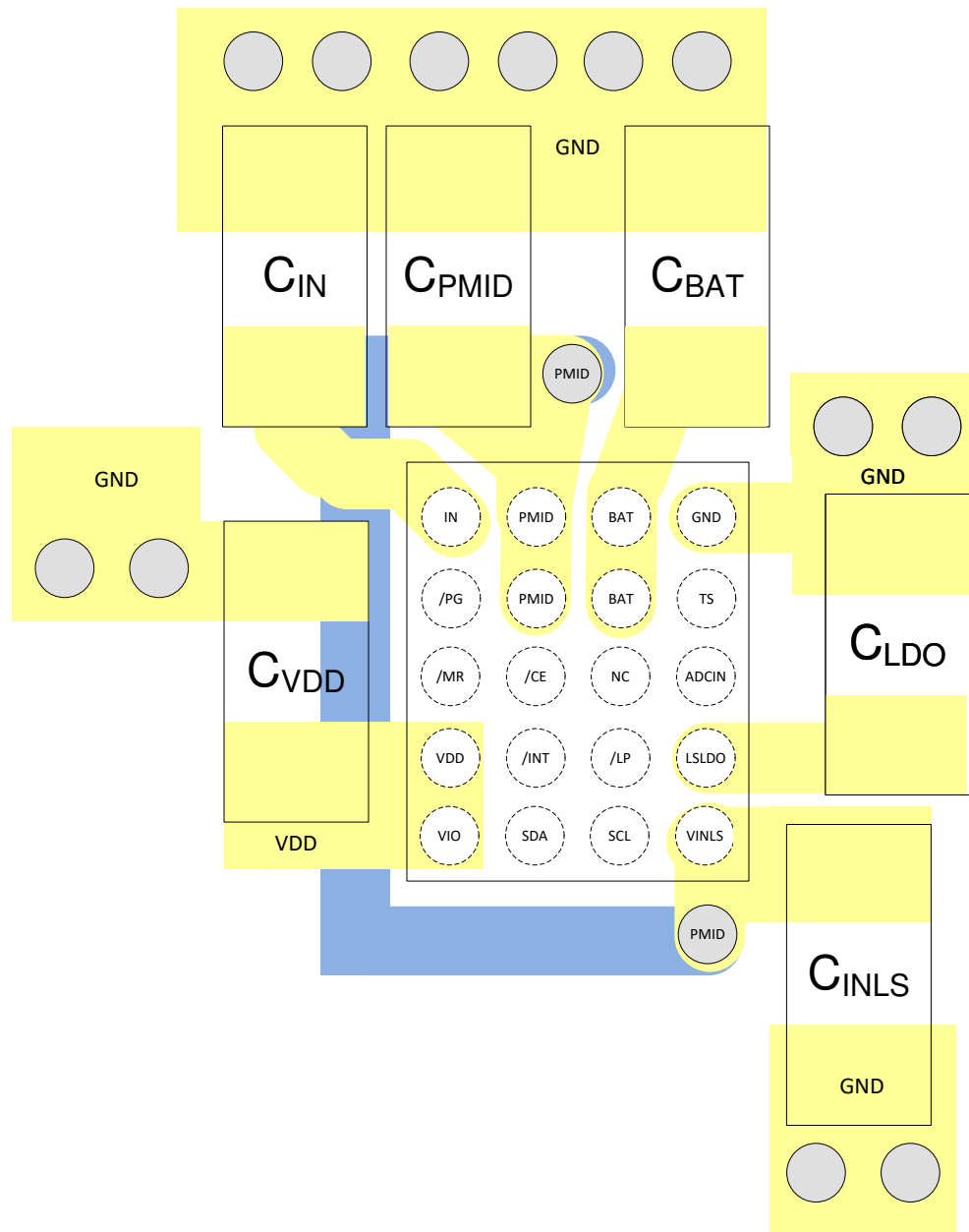
12-1. Layout Example
