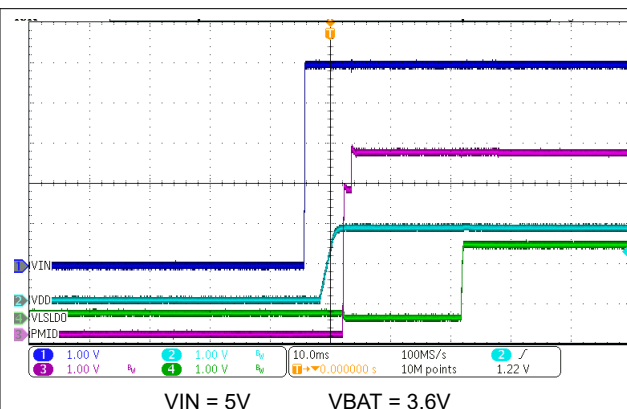
FIG 10-3. Power Up from Ship Mode with IN Supply Insertion
