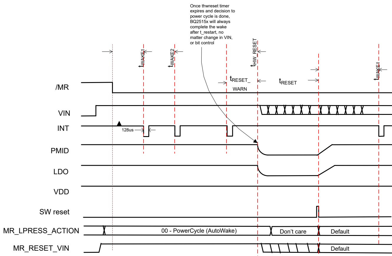
9-5. MR Wake and Reset Timing with VIN Present or BAT Active Mode When \text{MR\_LPRESS\_ACTION} = 00
