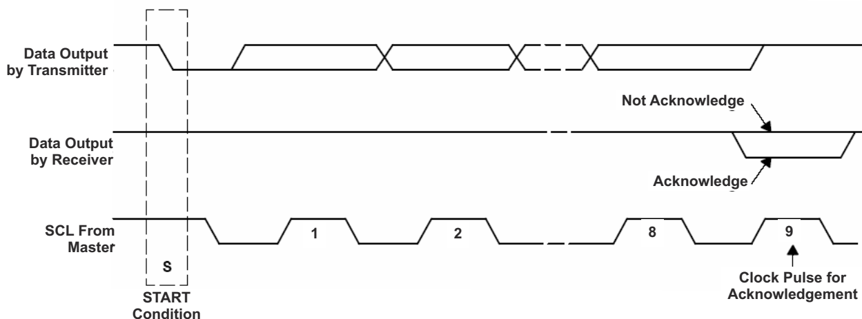
FIG 9-11. Acknowledge on the I 2 C Bus
