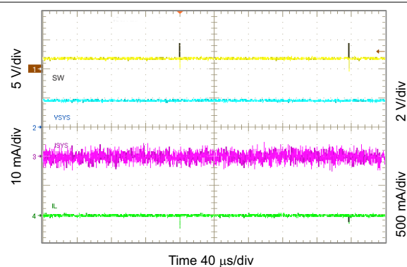
10-22. 3.3 V_{SYS} Line Regulation
