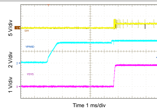
10-41. Startup Showing SS on SYS in PWM Mode
