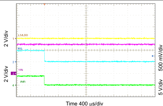
FIG 10-59. \overline{\text{PG}} Functions as Shifted \overline{\text{MR}} Output
