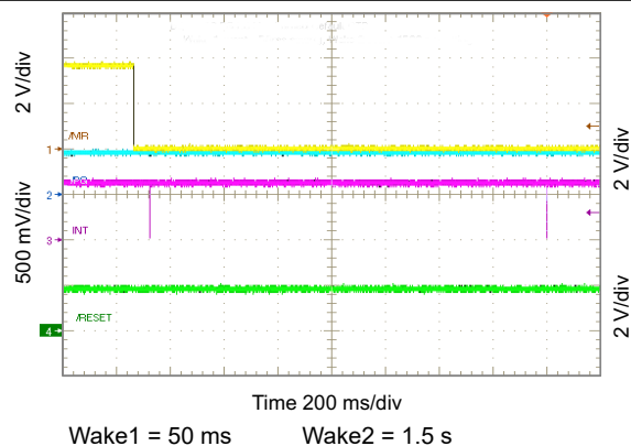
FIG 10-62. Show \overline{\text{MR}} Timing
