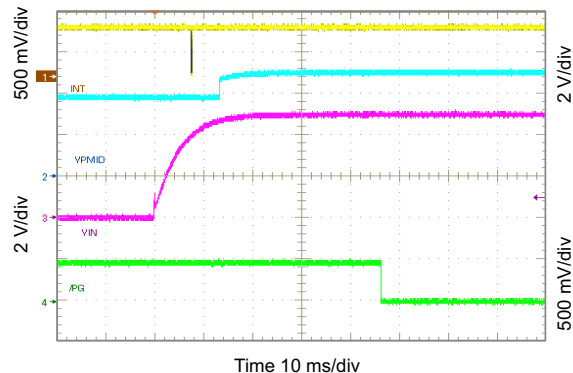
FIG 10-57. Show \overline{\text{PG}} and \overline{\text{INT}} Timing ( \text{VIN} Insertion)
