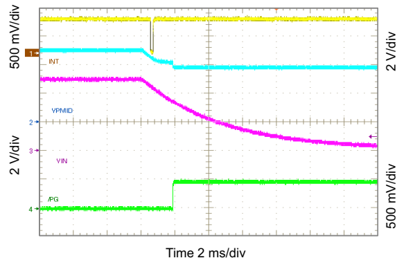
FIG 10-58. Show \overline{\text{PG}} and \overline{\text{INT}} Timing ( \text{VIN} Removal)
