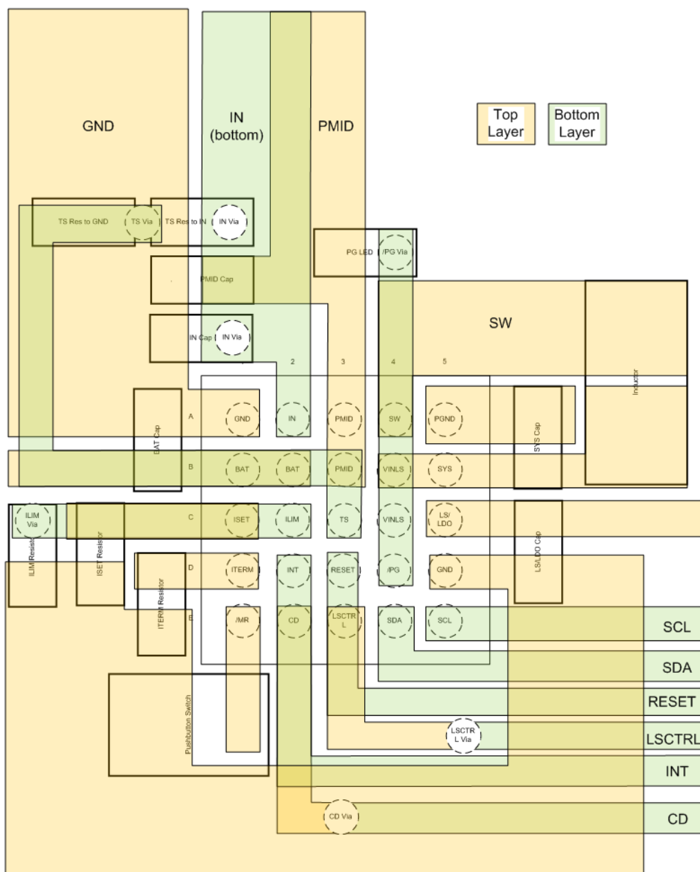
12-1. BQ25125 Layout
