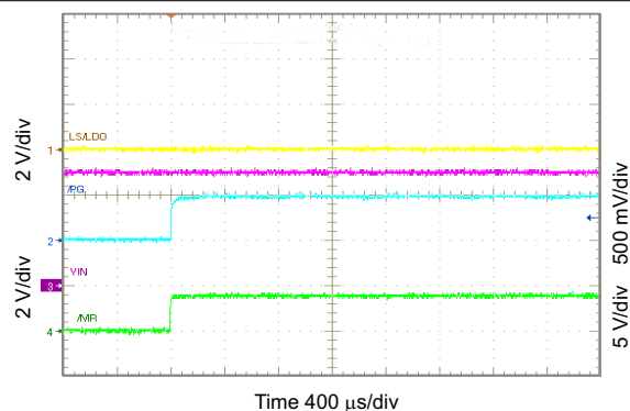
FIG 10-60. \overline{\text{PG}} Functions as Shifted \overline{\text{MR}} Output
