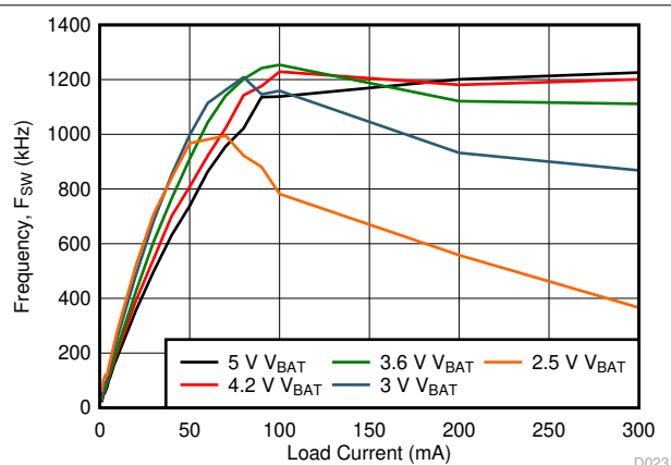
10-23. 1.8 V_{SYS} Switching Frequency vs Load Current
