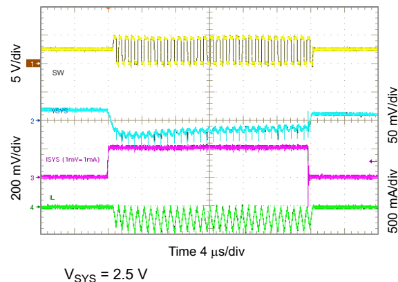
10-39. 2.5 V_{SYS} Load Transient, 0 to 200 mA
