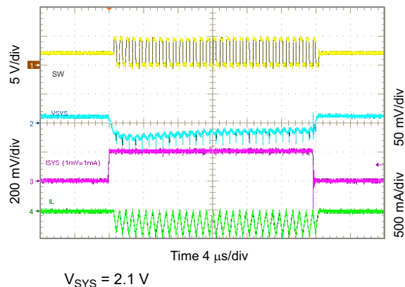
10-38. 2.1 V_{SYS} Load Transient, 0 to 200 mA
