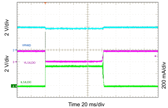
10-56. Short Circuit and Recovery for LDO
