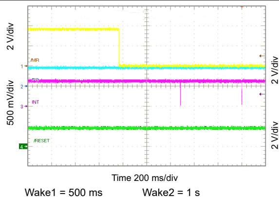
FIG 10-61. Show \overline{\text{MR}} Timing
