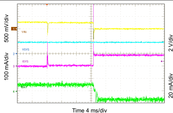
FIG 10-6. Entering Battery Supplement Mode
