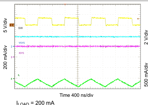
10-31. Light Load Operation Showing SW
