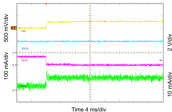
FIG 10-5. Exiting DPPM Mode
