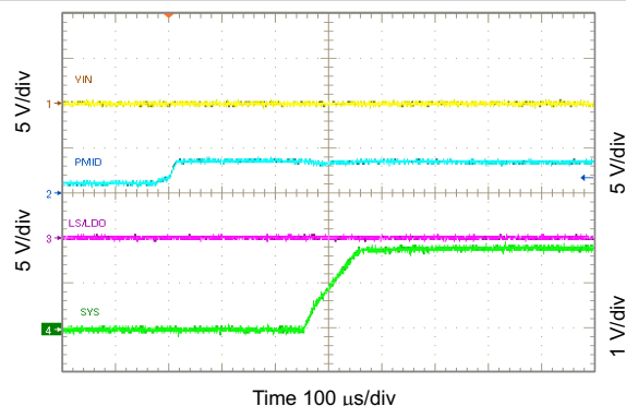
FIG 10-2. Battery Connected to V_{(BAT)}
