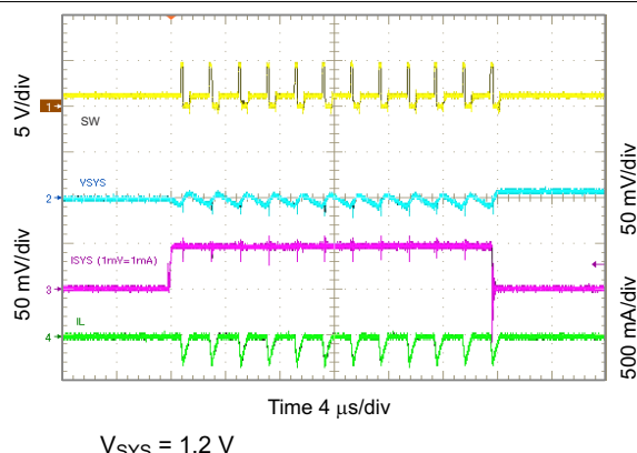
10-33. 1.2 V_{SYS} Load Transient, 0 to 50 mA
