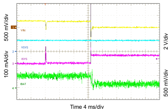
FIG 10-4. Entering DPPM Mode
