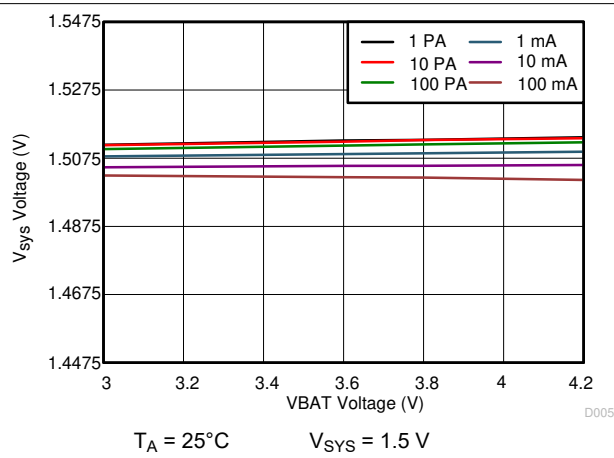
10-21. 1.5 V sys Line Regulation
