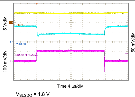
10-54. 1.8 V_{\text{LSLDO}} Load Transient, 0 to 100 mA
