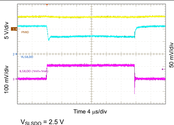
10-55. 2.5 V_{\text{LSLDO}} Load Transient, 0 to 100 mA
