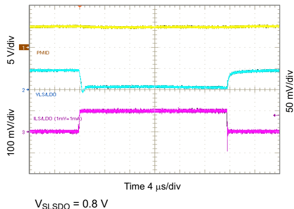
10-52. 0.8 V_{\text{LSLDO}} Load Transient, 0 to 100 mA
