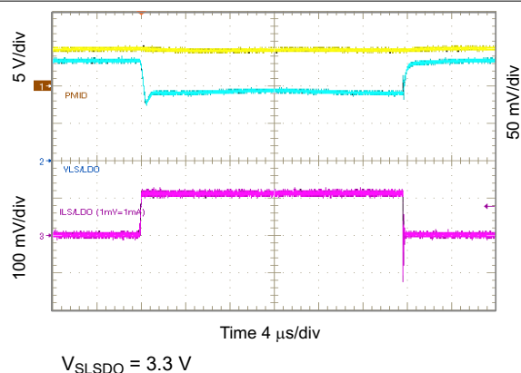
10-56. 3.3 V_{\text{LSLDO}} Load Transient, 0 to 100 mA
