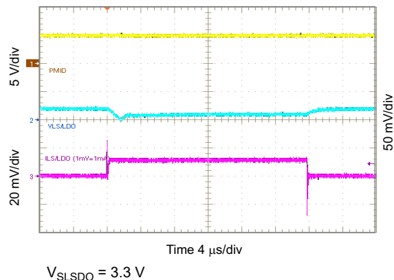
10-51. 3.3 V_{\text{LSLDO}} Load Transient, 0 to 10 mA
