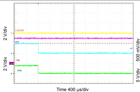
10-61. \overline{PG} Functions as Shifted \overline{MR} Output
