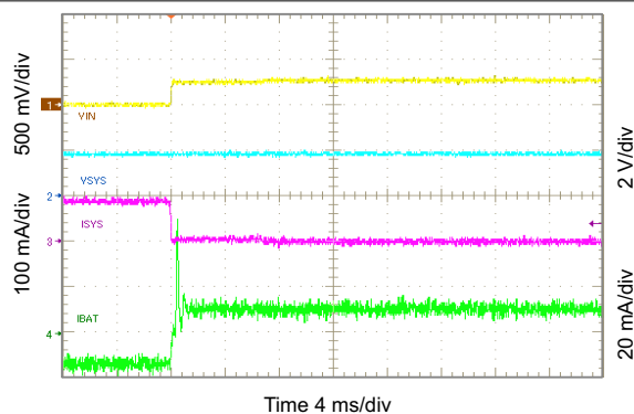
FIG 10-7. Exiting Battery Supplement Mode
