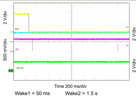
10-64. Show \overline{MR} Timing
