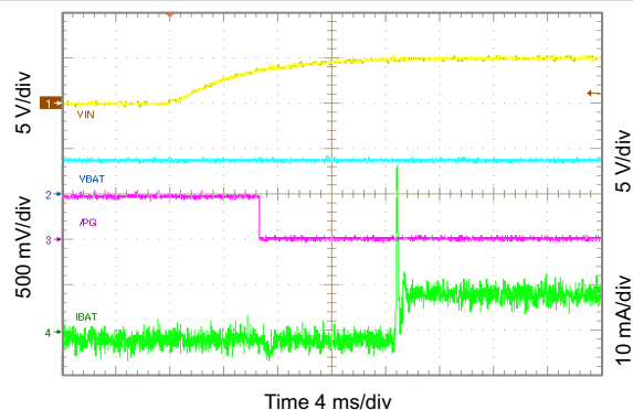
FIG 10-3. Power Supply Connected to V_{IN}
