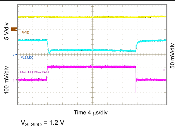
10-53. 1.2 V_{\text{LSLDO}} Load Transient, 0 to 100 mA
