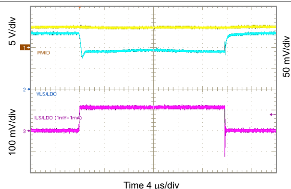
90. 1.8 V_{SLSDO} Load Transient, 0 to 100 mA
