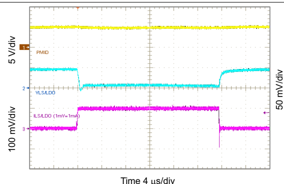
88. 0.8 V_{SLSDO} Load Transient, 0 to 100 mA
