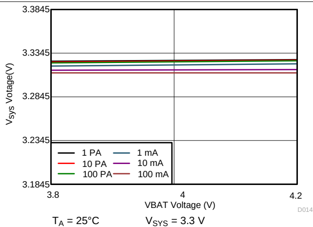
60. 3.3 V SYS Line Regulation
