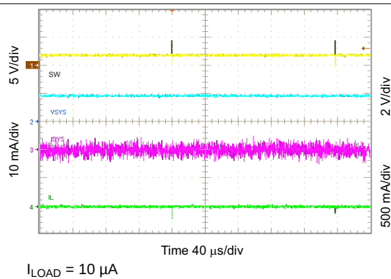
62. Light Load Operation Showing SW
