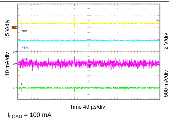
63. Light Load Operation Showing SW
