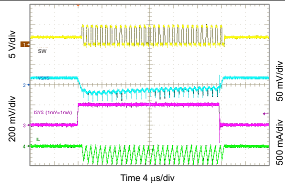
Figure 75. 1.8 V SYS Load Transient, 0 to 200 mA
