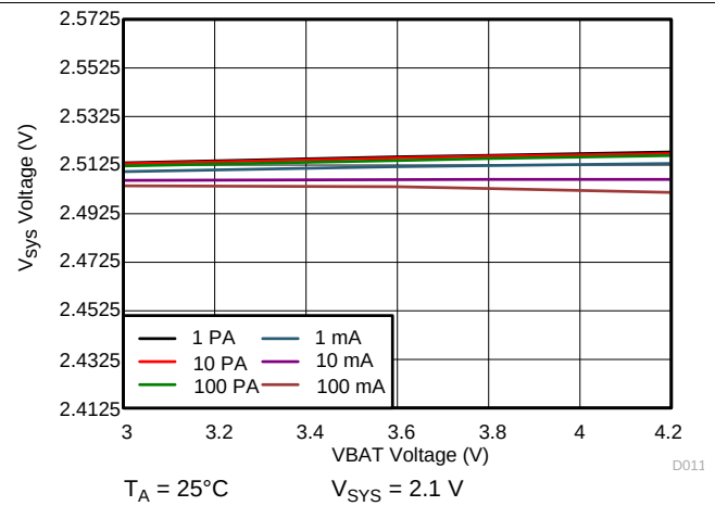
59. 2.1 V SYS Line Regulation
