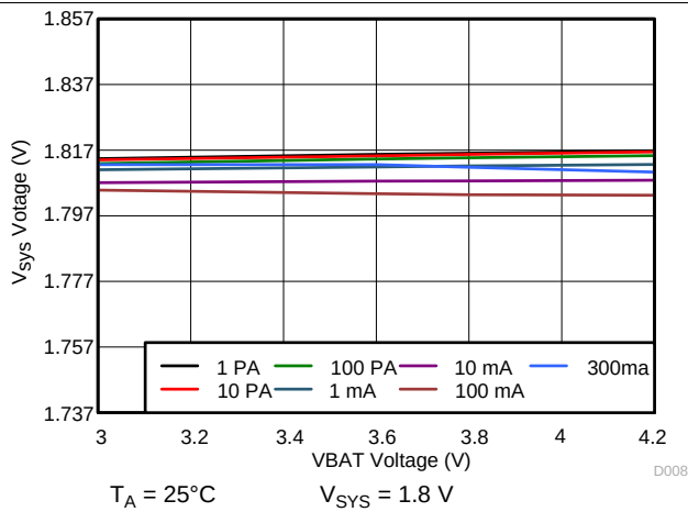
58. 1.8 V SYS Line Regulation
