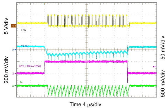
Figure 74. 1.2 V SYS Load Transient, 0 to 200 mA
