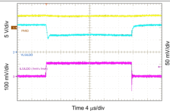
89. 1.2 V_{SLSDO} Load Transient, 0 to 100 mA
