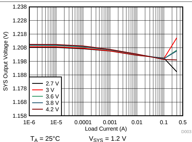
FIG 49. 1.2 V SYS Load Regulation
