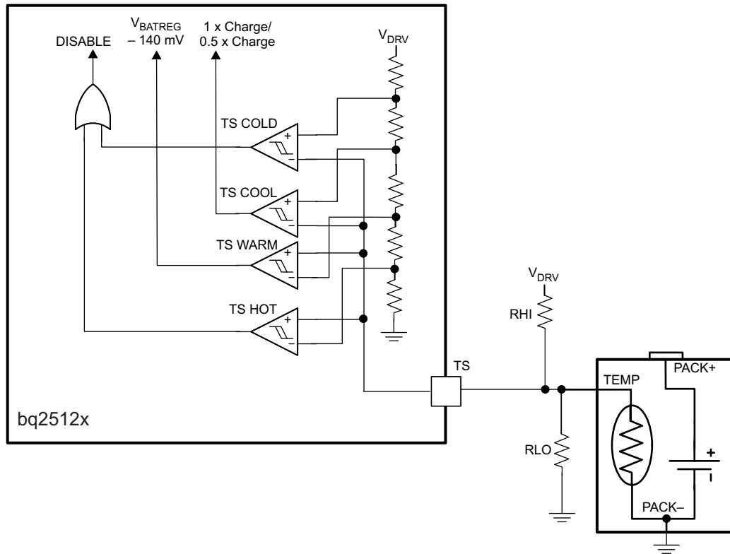
FIG 16. TS Circuit
