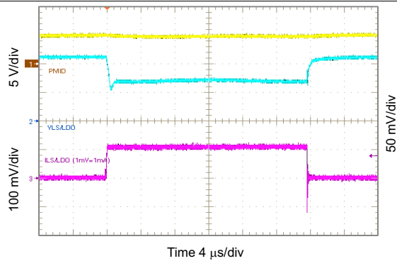
87. 1.2 V_{SLSDO} Load Transient, 0 to 100 mA
