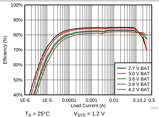
FIG 44. 1.2 V SYS System Efficiency
