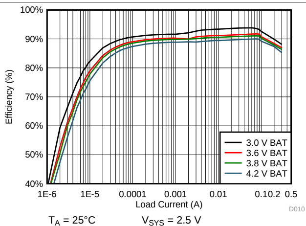
FIG 47. 2.5 V SYS System Efficiency
