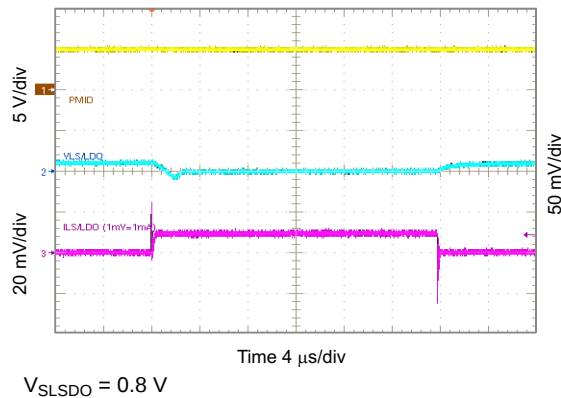
图 81. 0.8 V_{LSLDO} Load Transient, 0 to 10 mA
