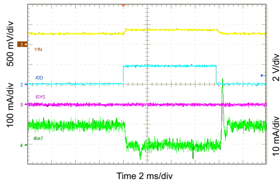
图 42. Charger On/Off Using \overline{CD}
