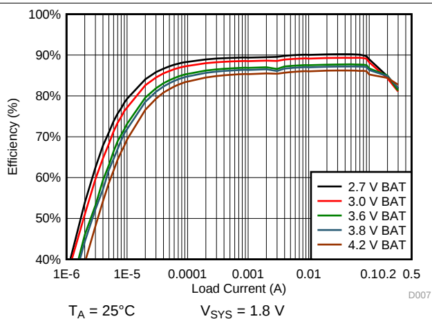
FIG 46. 1.8 V SYS System Efficiency
