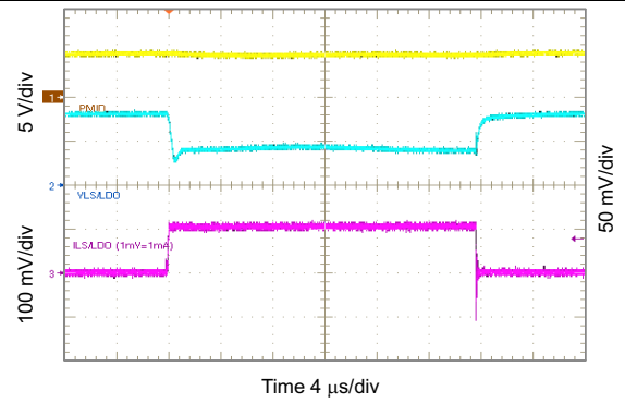
86. 0.8 V_{SLSDO} Load Transient, 0 to 100 mA
