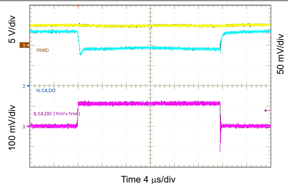
88. 1.8 V_{SLSDO} Load Transient, 0 to 100 mA
