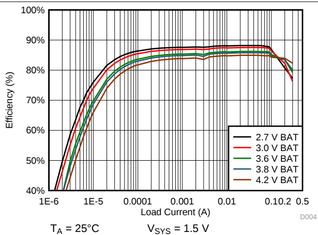
FIG 45. 1.5 V SYS System Efficiency
