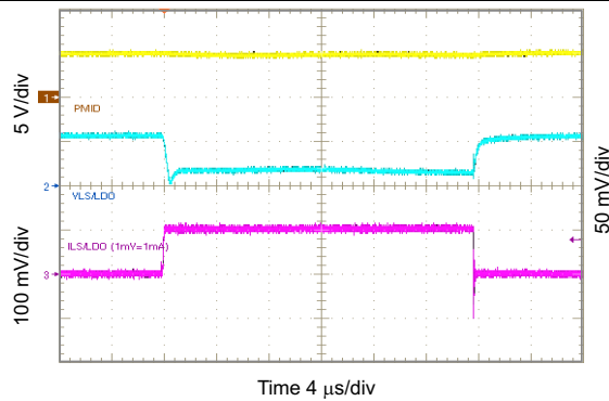
85. 3.3 V_{SLSDO} Load Transient, 0 to 10 mA
