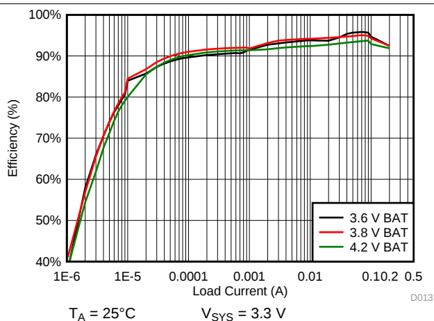
FIG 48. 3.3 V SYS System Efficiency
