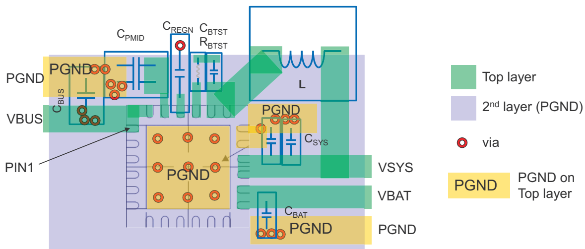
12-2. Layout Example
