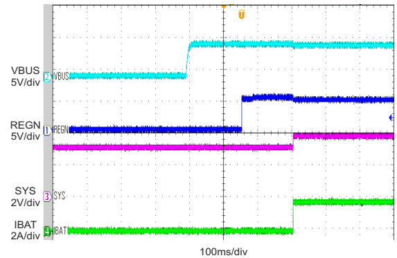
10-4. BQ24297 Power Up with Charge Enabled
