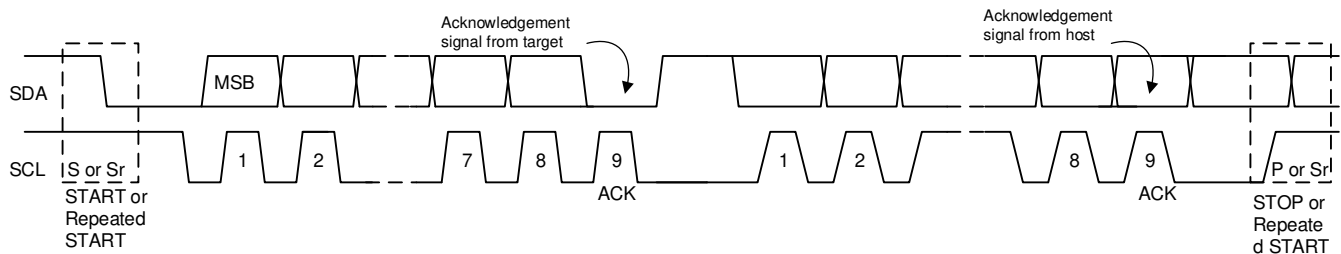
FIG 9-13. Data Transfer on the I 2 C Bus
