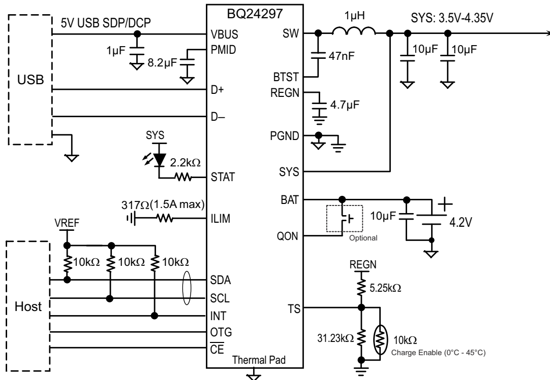
10-2. BQ24297 with USB D+/D- Detection, USB On-The-Go (OTG) and Optional BATFET Enable Interface
