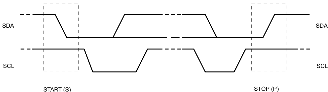
FIG 9-12. START and STOP Conditions
