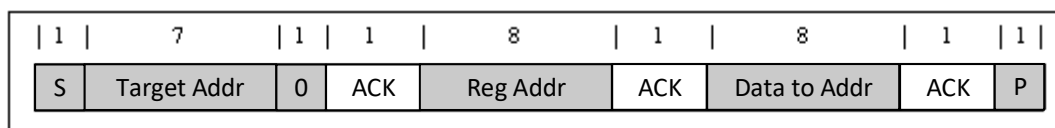
FIG 9-15. Single Write
