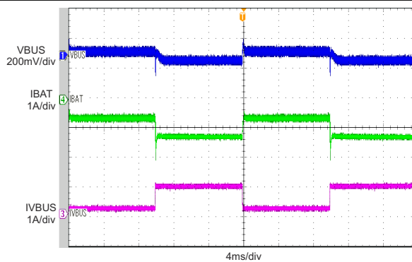
10-11. Load Transient During Supplement Mode
