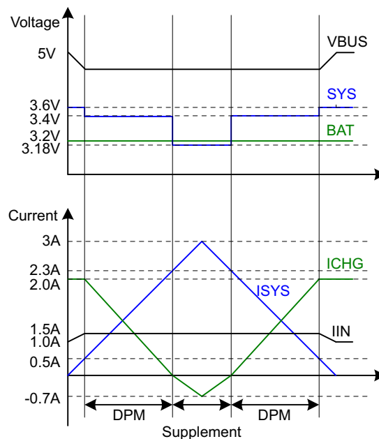
9-4. DPM Response
