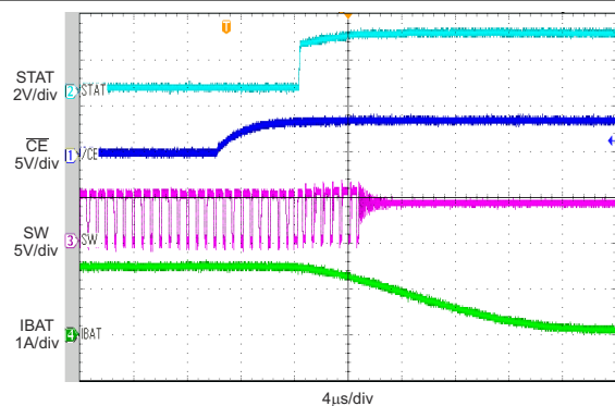
10-7. Charge Disable
