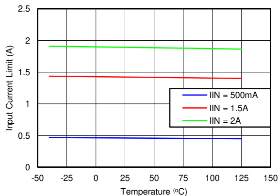
8-9. Input Current Limit vs Temperature
