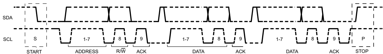
FIG 9-14. Complete Data Transfer
