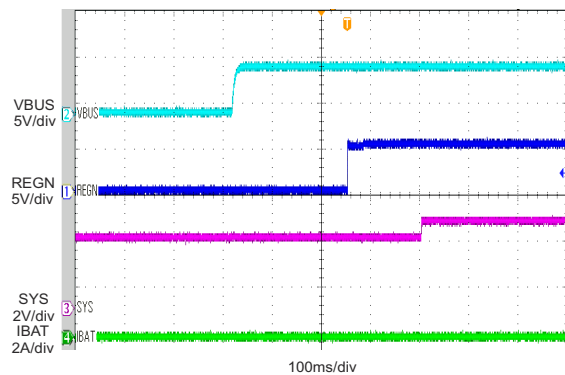
10-3. BQ24296 Power Up with Charge Enabled
