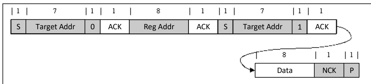
FIG 9-16. Single Read
