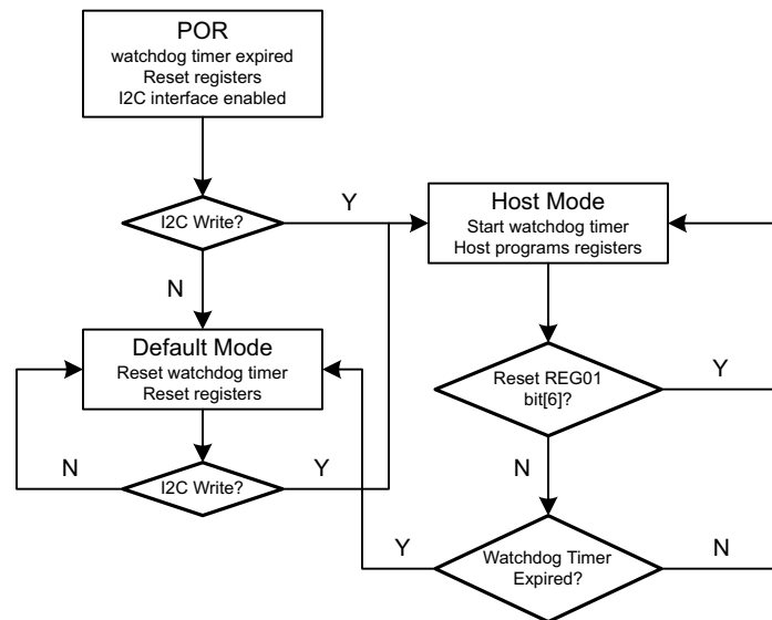
9-10. Watchdog Timer Flow Chart
