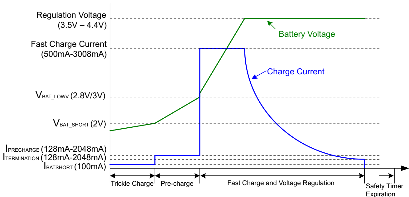
図 9-6. Battery Charging Profile
