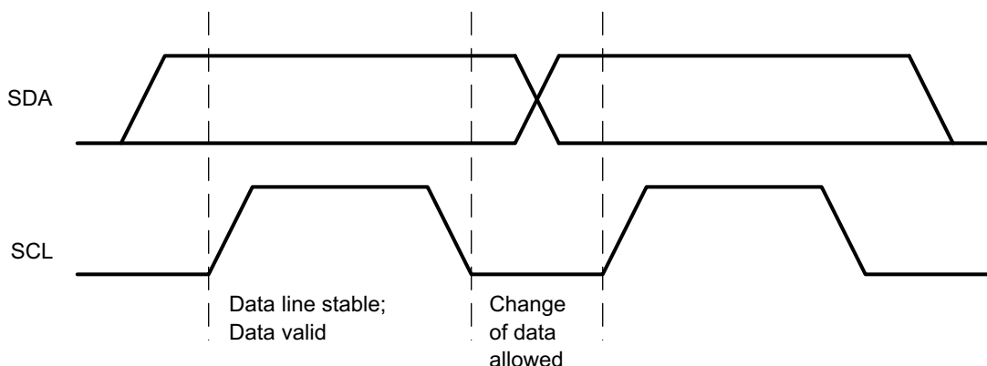
FIG 9-11. Bit Transfer on the I 2 C Bus
