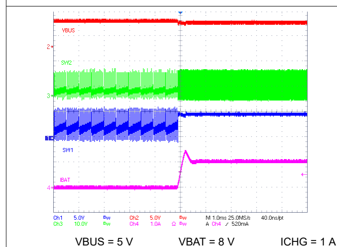
9-5. Charge Enable
