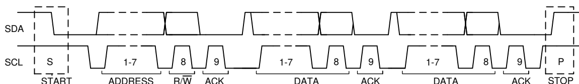
FIG 8-17. Complete Data Transfer on the I 2 C Bus
