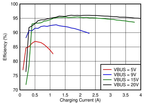
7-1. 2s Battery Charge Efficiency vs. Charge Current
