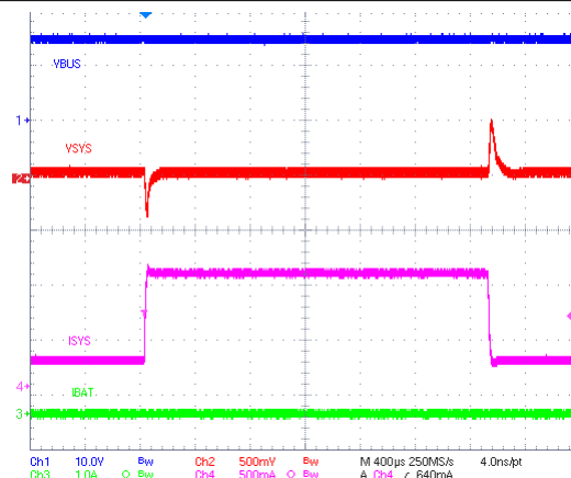
9-10. Buck Mode PFM with OOA
