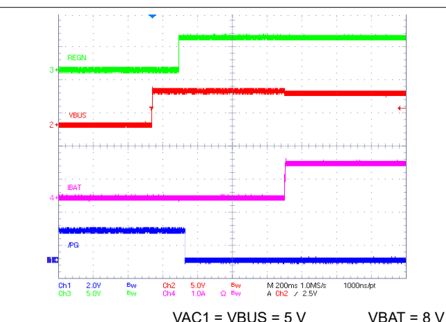
9-4. Power Up from VAC1 with Charge Enabled
