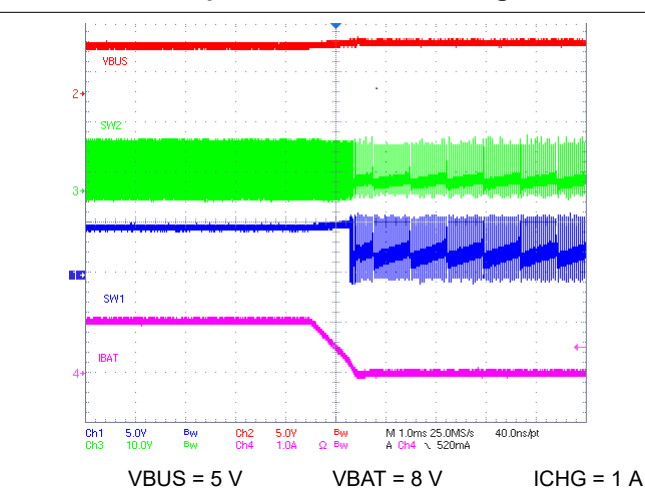
9-6. Charge Disable
