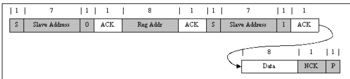
FIG 8-19. Single Read
