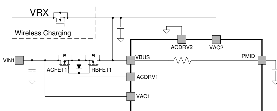
FIG 8-2. One ACFET-RBFET Structure Supporting One Input at VAC1 and/or One Input at VBUS
