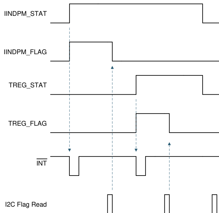
FIG 8-11. INT Generation Behavior Example
