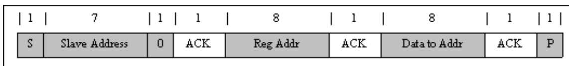
FIG 8-18. Single Write
