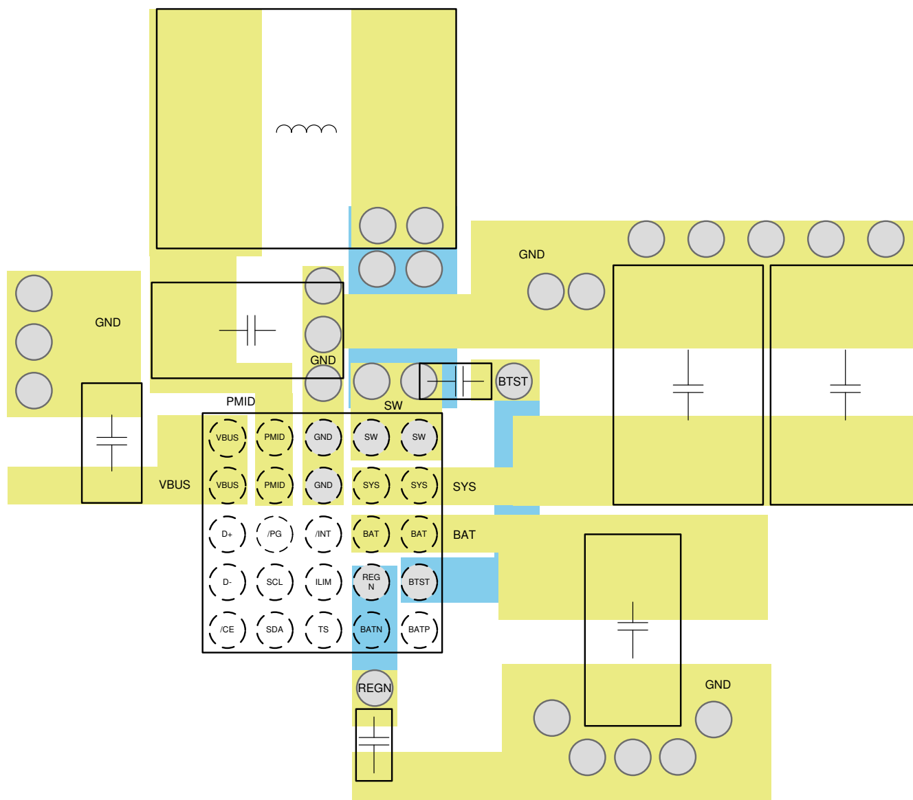
11-2. PCB Layout Example
