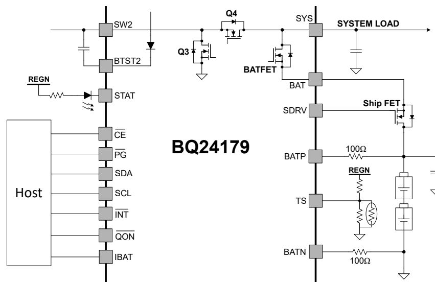
FIG 8-12. The Application Diagram for the External Ship FET
