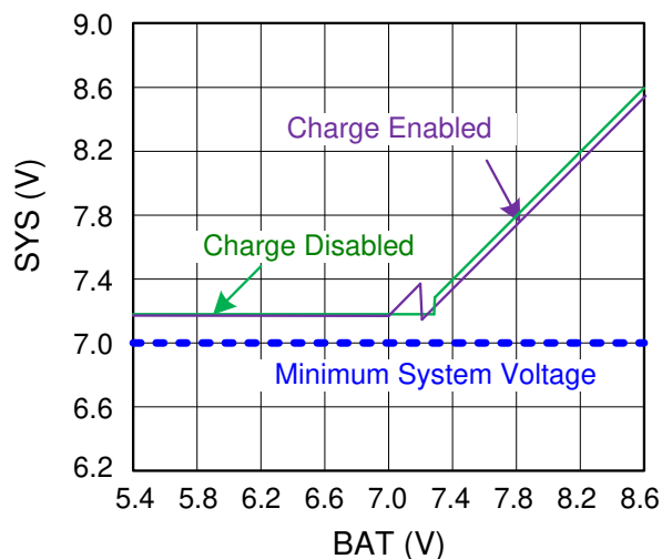
✎ 8-6. Typical System Voltage vs Battery Voltage for a 2S Battery Configuration
