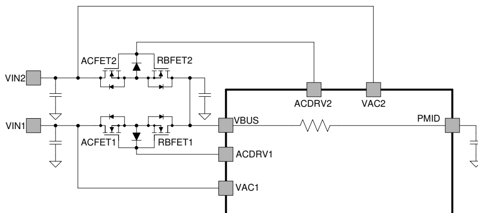
FIG 8-3. Two ACFETs-RBFETs Structure Supporting One Input at VAC1 and One Input at VAC2
