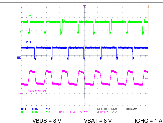
9-8. Buck-Boost Charging Mode PWM Operation
