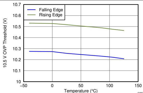
FIG 7-7. 10.5-V OVP Threshold vs Temperature
