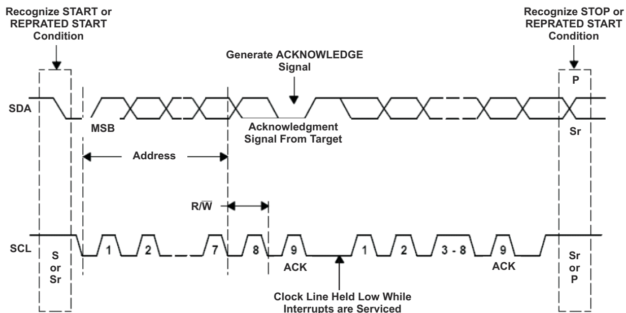
Figure 8-11. Bus Protocol
