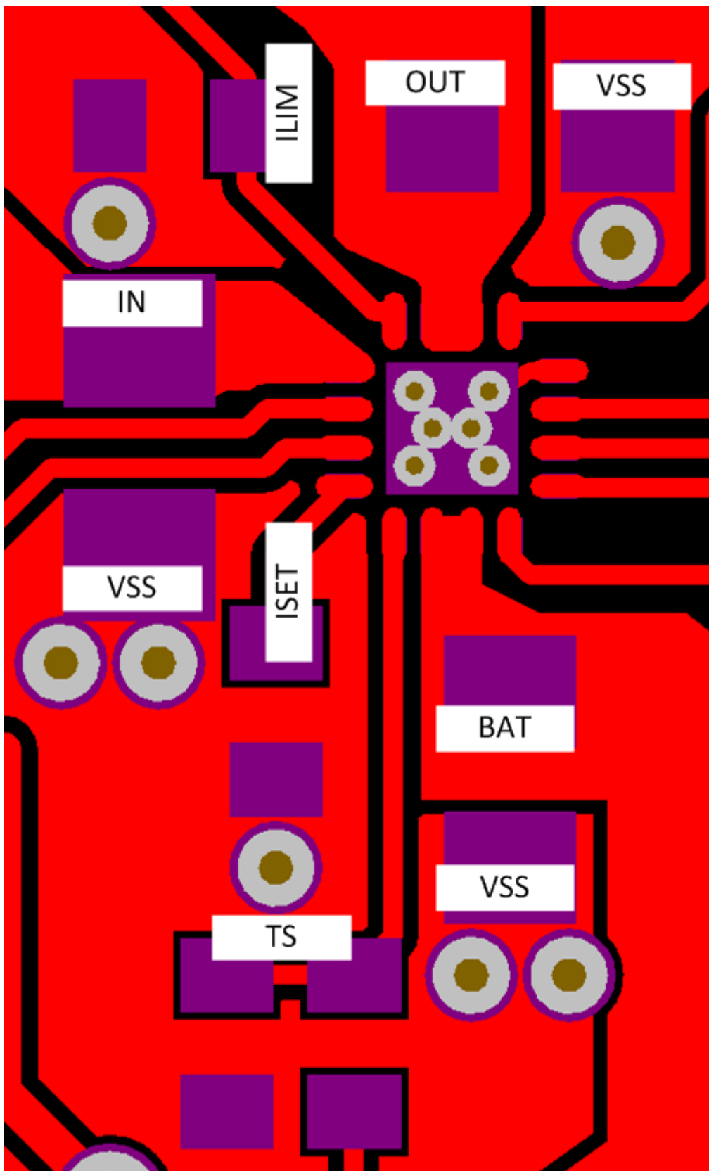
12-1. Layout Schematic
