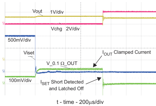
9-14. ISET Shorted During Normal Operation
