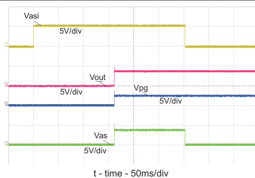
9-24. ASI and Delayed OUT Power-up Timing – No Input, BQ24041
