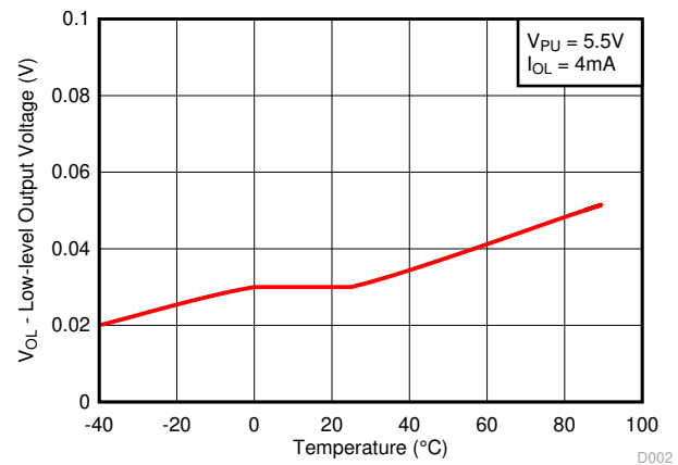
Figure 6-2. Low-Level Output Voltage vs Temperature
