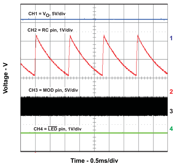
Figure 15. bq2000T in Fast Charge
