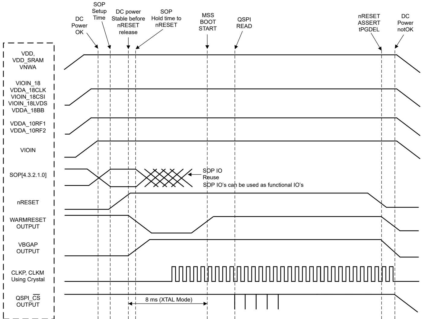
図 7-2. Device Wake-up Sequence
