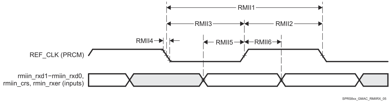
图 7-15. MAC Receive Interface Timing, RMII operation
