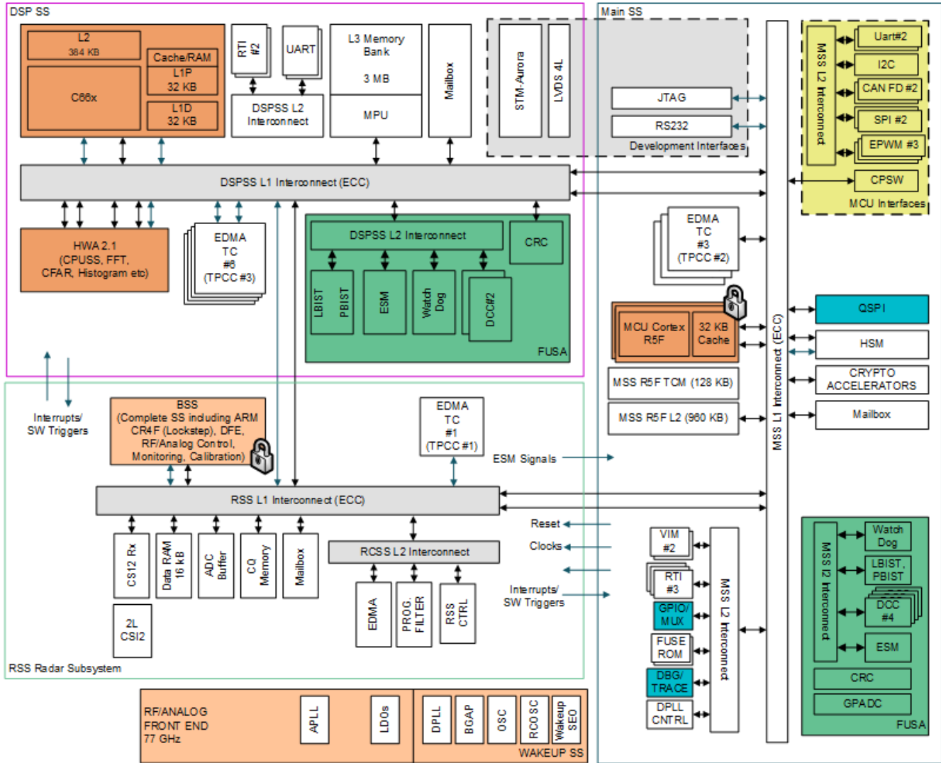
図 8-5. Processor Subsystem
