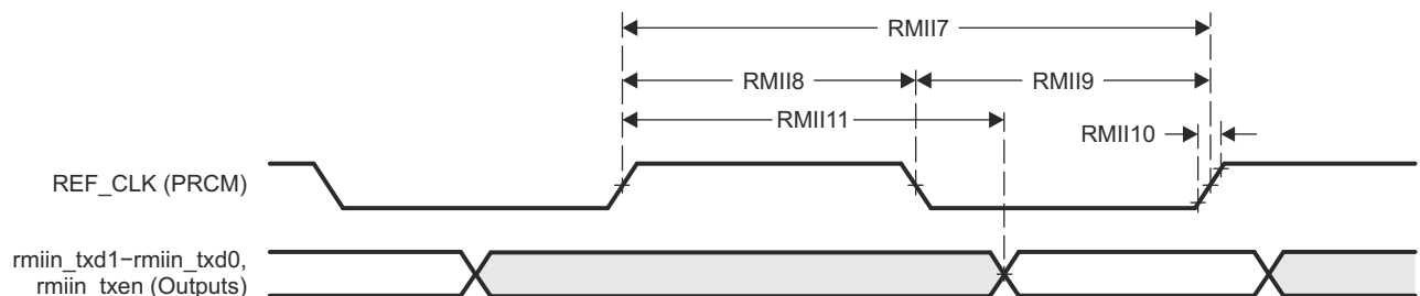
FIG 7-14. MAC Transmit Interface Timing, RMII operation
