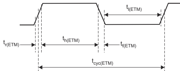
図 7-25. ETMTRACECLKOUT Timing
