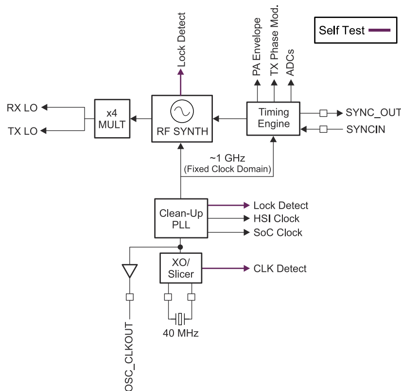
☒ 7-2. RF Clock Subsystem
