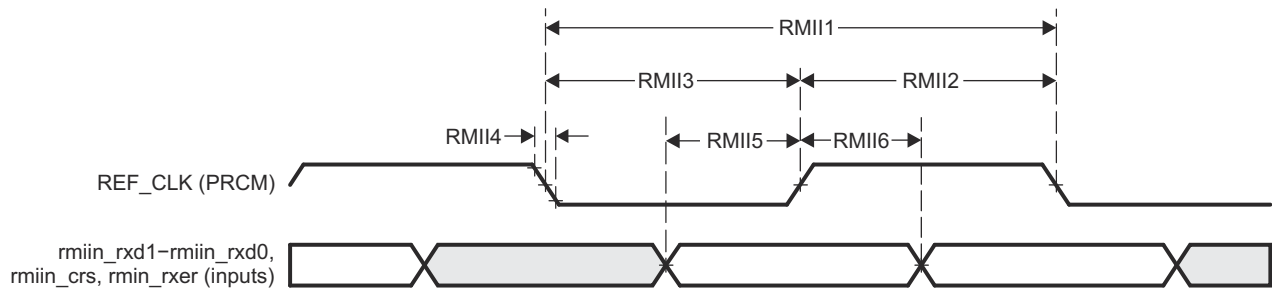
图 6-15. MAC Receive Interface Timing, RMII operation
