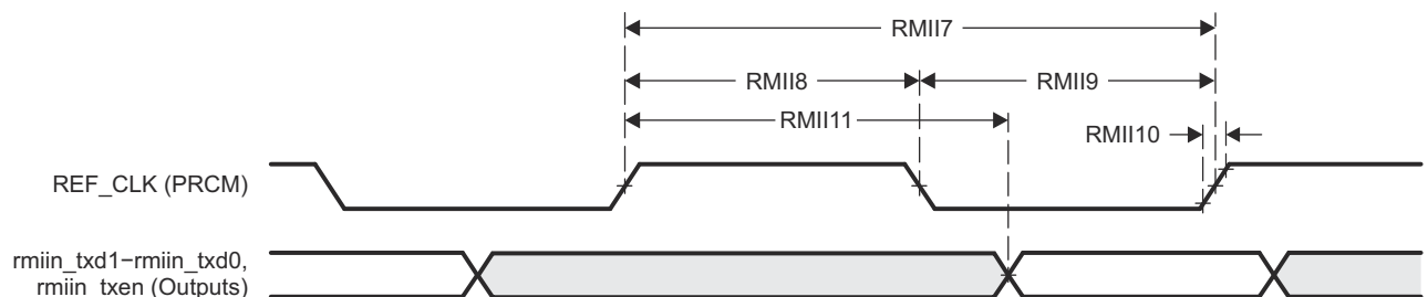
图 6-14. MAC Transmit Interface Timing, RMII operation
