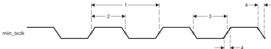
図 6-19. Clock Timing (MAC Transmit) - MII operation
