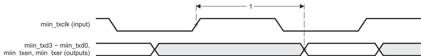
图 6-16. MAC Transmit Interface Timing, MII operation
