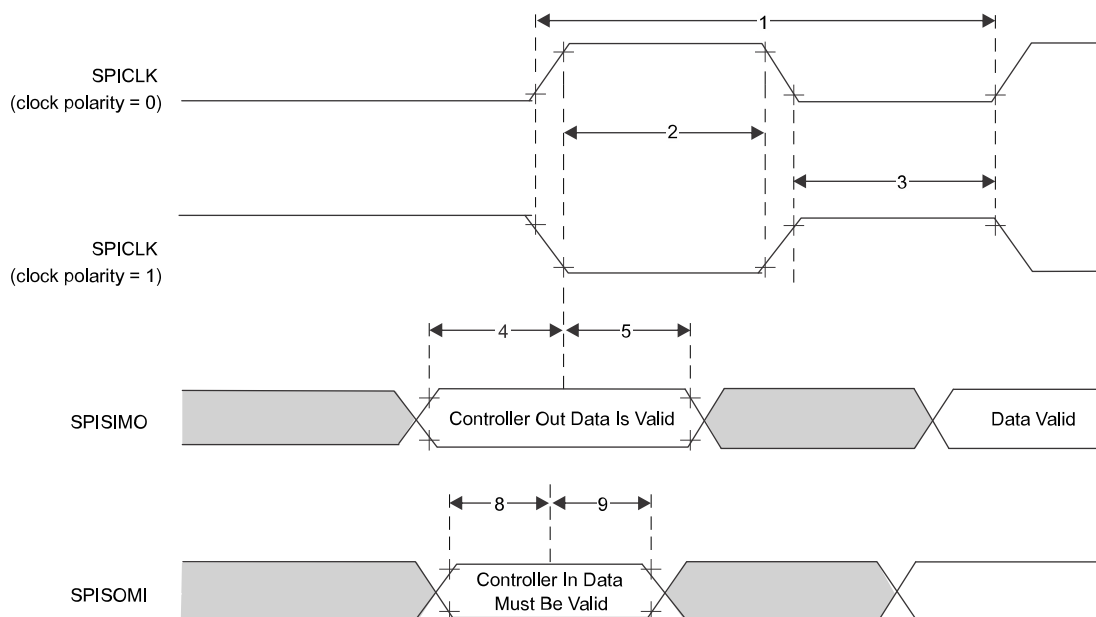
図 6-8. SPI Controller Mode External Timing (CLOCK PHASE = 1)
