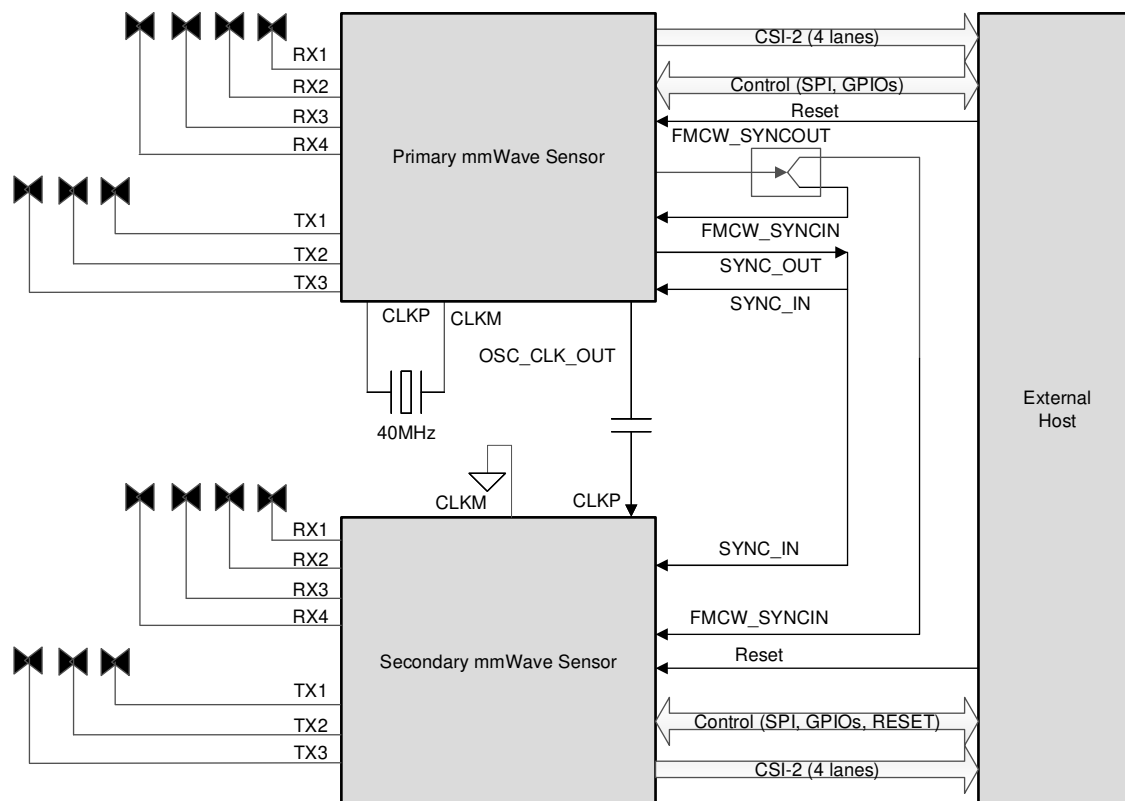
10-2. Imaging Radar using Cascade Configuration
