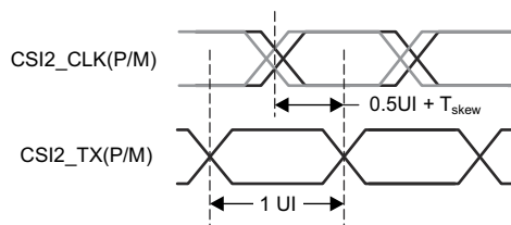
図 7-10. Clock and Data Timing in HS Transmission
