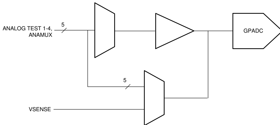
7-5. ADC Path
