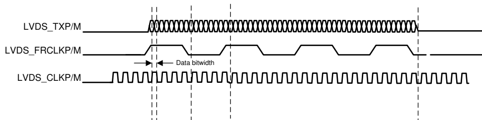
❏ 6-15. LVDS Interface Lane Configuration And Relative Timings
