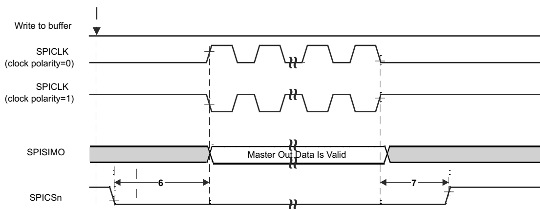
8-8. SPI Controller Mode Chip Select Timing (CLOCK PHASE = 1)
