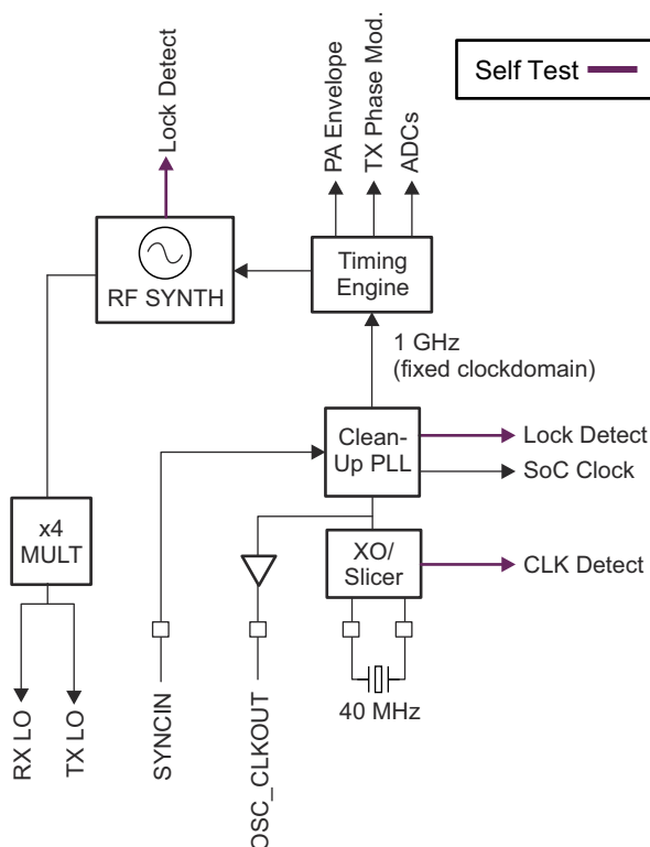
Figure 9-3. Clock Subsystem
