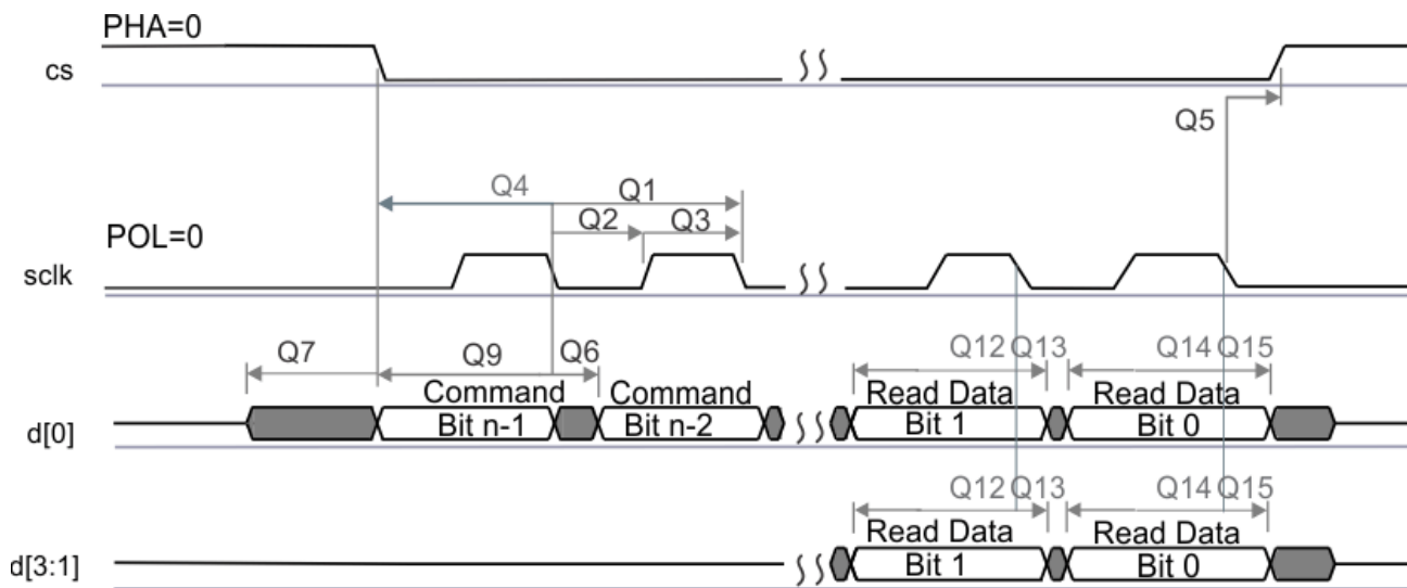
✎ 8-15. QSPI Read (Clock Mode 0)
