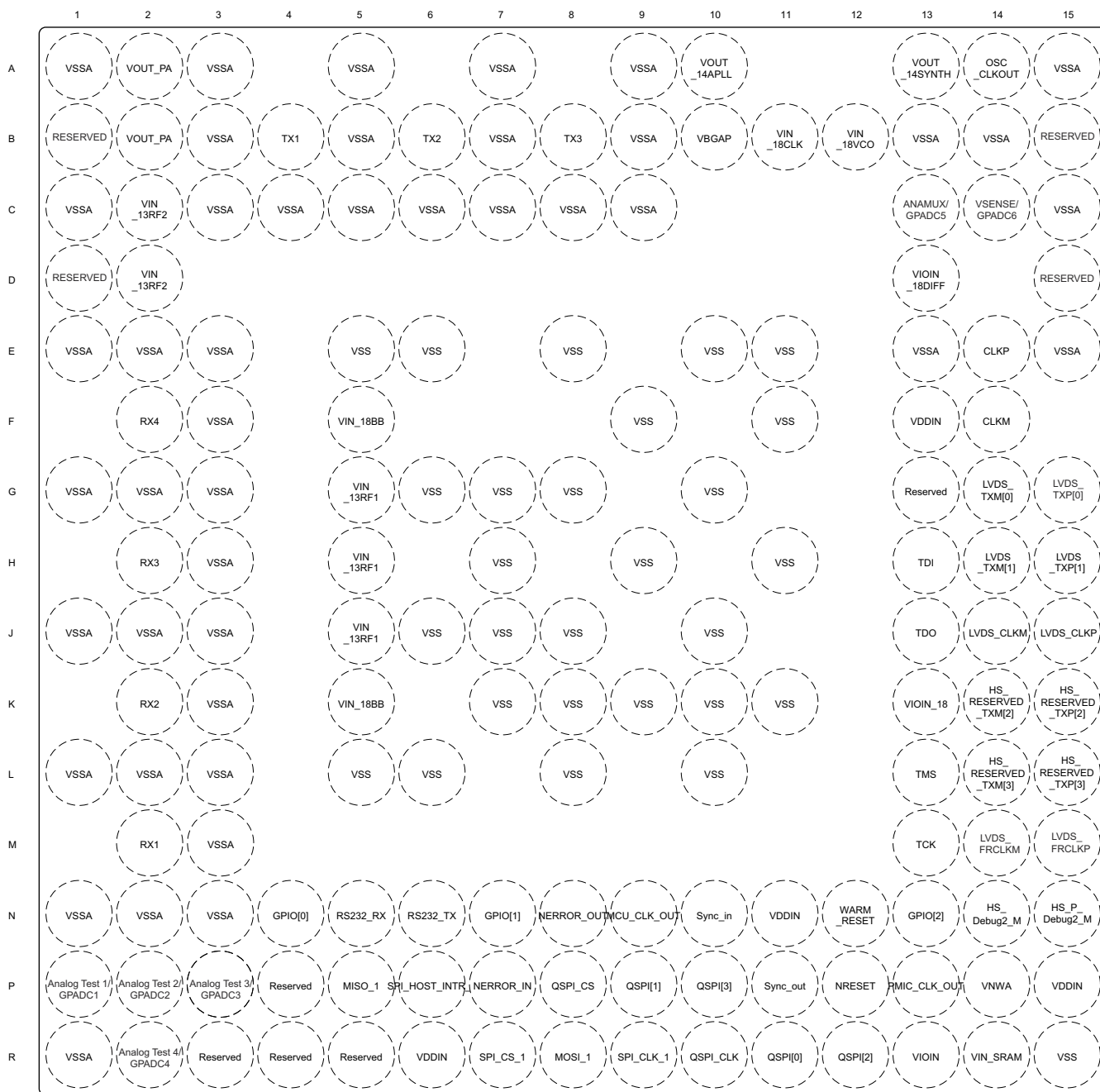
Figure 7-1. Pin Diagram
