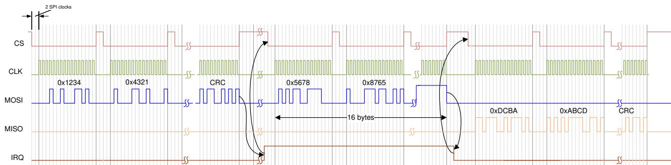
Figure 8-11. SPI Communication
