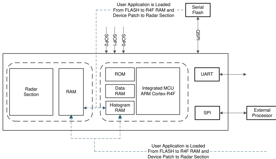
9-8. Bootloader's Functional Mode
