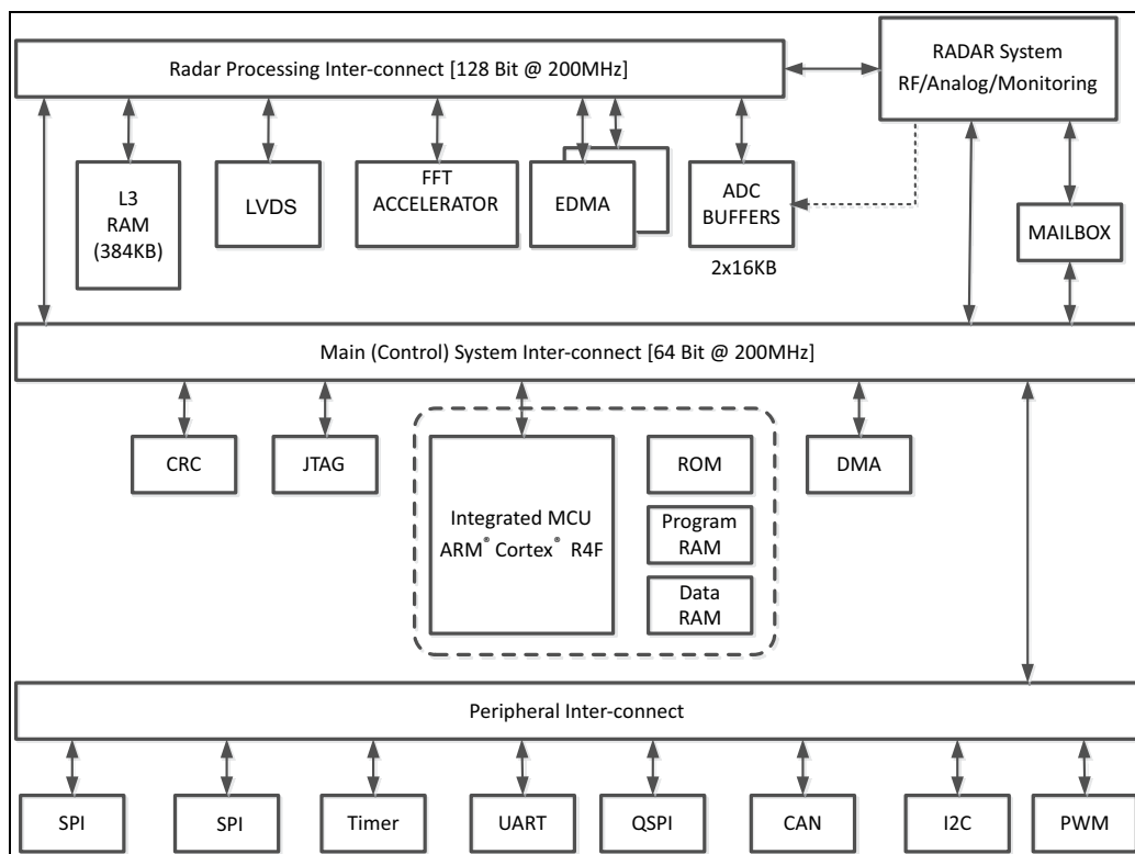
❏ 9-2. System Interconnect
