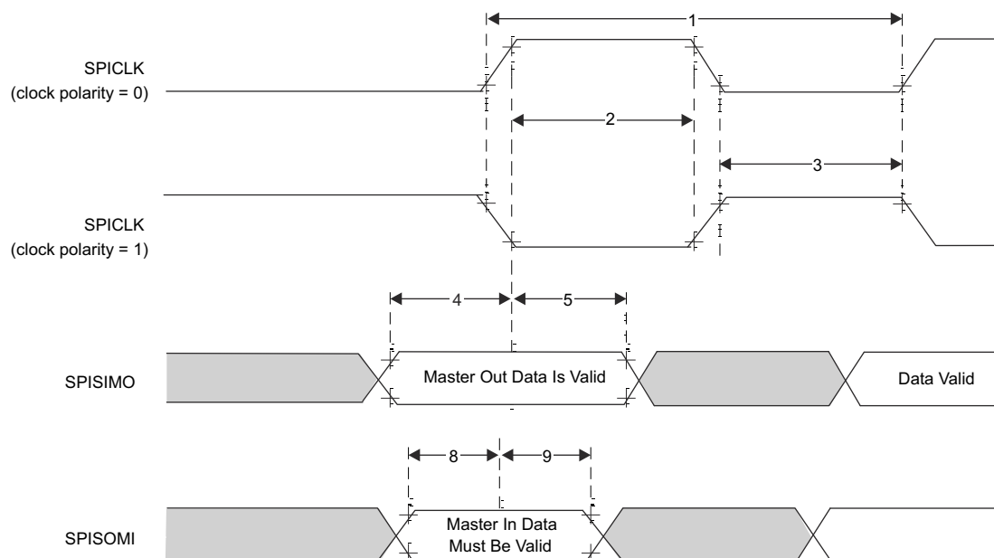
8-7. SPI Controller Mode External Timing (CLOCK PHASE = 1)
