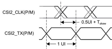
図 8-9. Clock and Data Timing in HS Transmission
