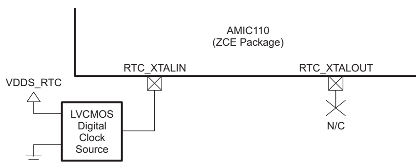
Figure 6-15. OSC1 (ZCE Package) LVC MOS Circuit Schematic
