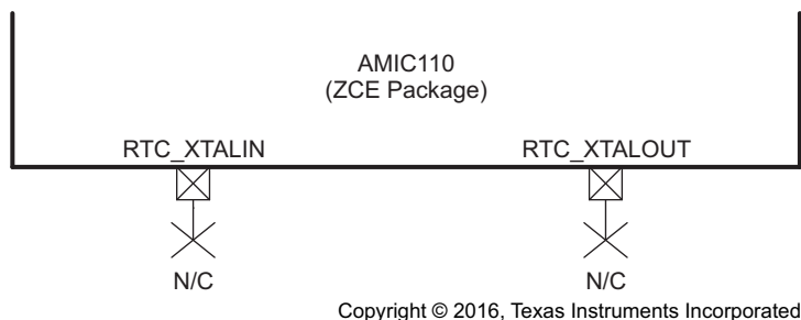
✕ 6-17. OSC1 (ZCE Package) Not Used Schematic
