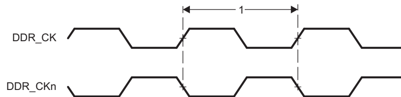
図 7-32. LPDDR Memory Interface Clock Timing
