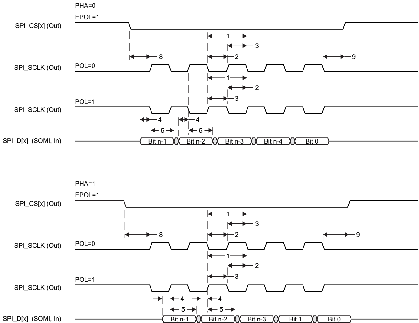
7-75. SPI Master Mode Receive Timing
