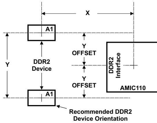
Figure 7-41. AMIC110 Device and DDR2 Device Placement
