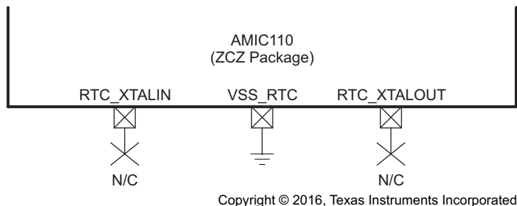
✕ 6-18. OSC1 (ZCZ Package) Not Used Schematic
