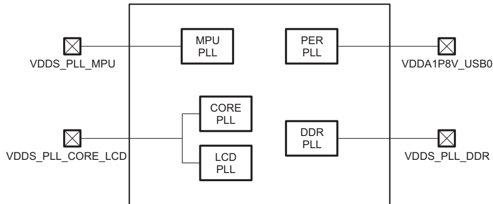
図 6-8. DPLL Power Supply Connectivity
