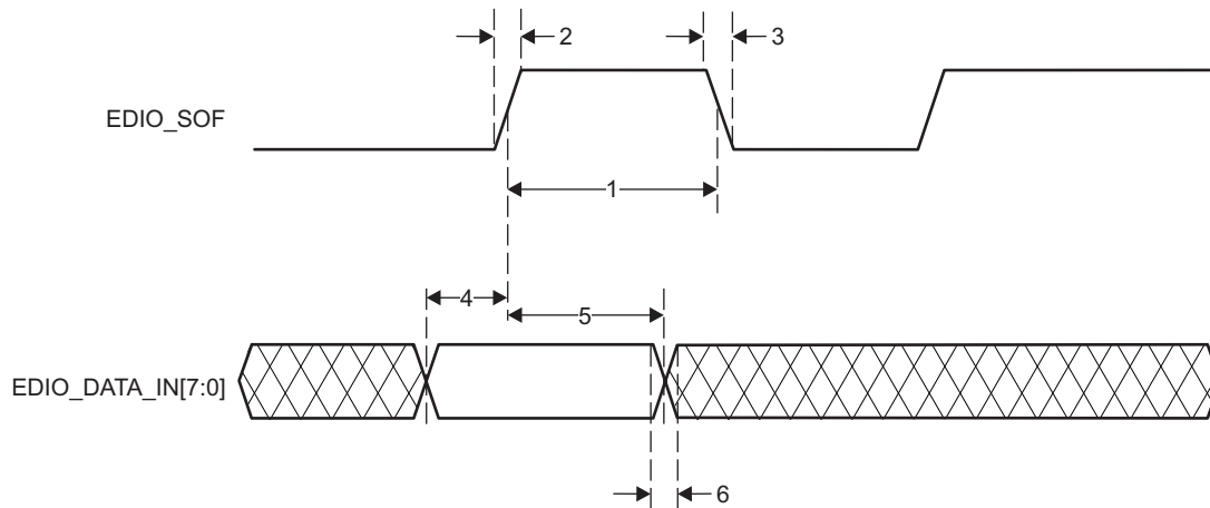
図 7-89. PRU-ICSS ECAT Input Validated With SOF
