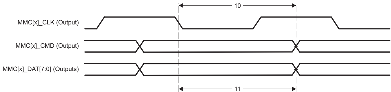
図 7-79. MMC[x]_CMD and MMC[x]_DAT[7:0] Output Timing—Standard Mode
