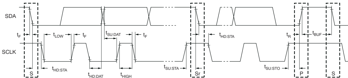
7-1. Timing Specification
