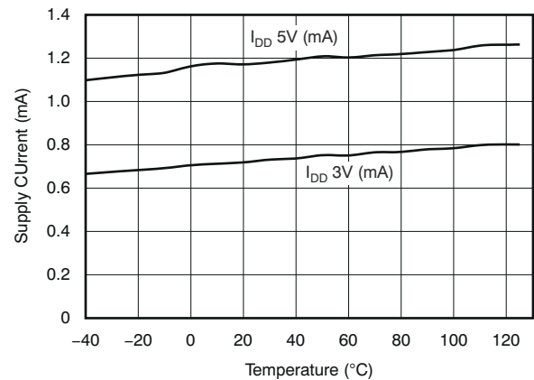
FIG 7-7. Supply Current vs Temperature
