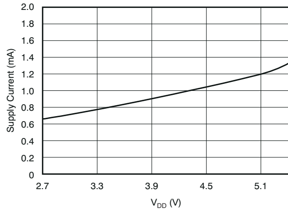
FIG 7-6. Supply Current vs V DD
