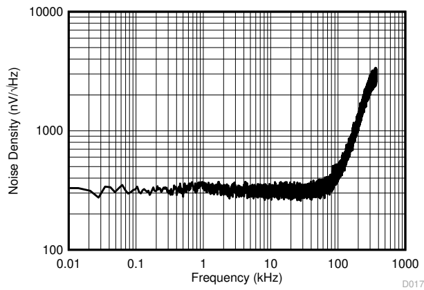
図 5-29. Input-Referred Noise Density vs Frequency
