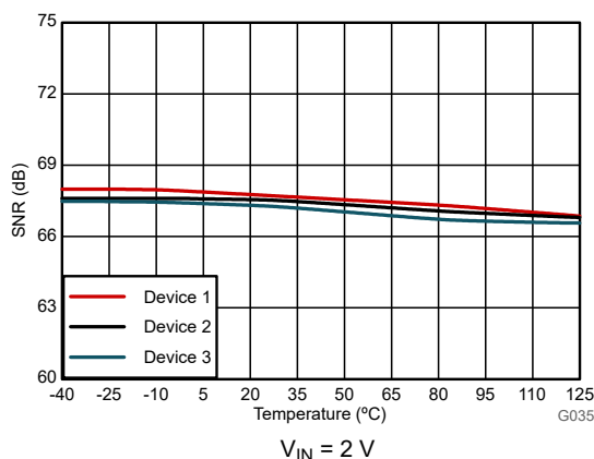
FIG 6-25. Signal-to-Noise Ratio vs Temperature
