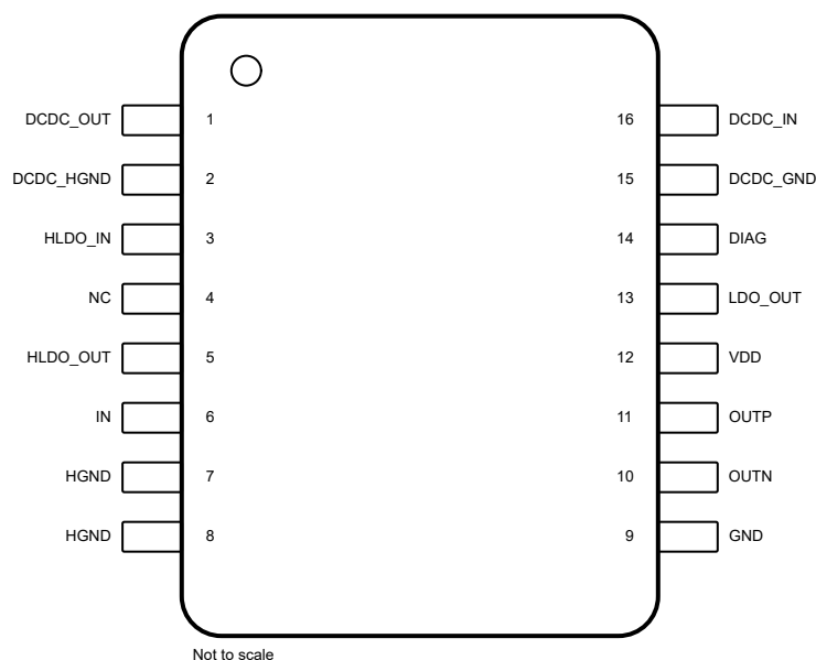
図 5-1. DWE Package, 16-Pin SOIC (Top View)
