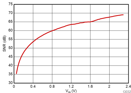
FIG 6-23. Signal to Noise Ratio vs Input Voltage
