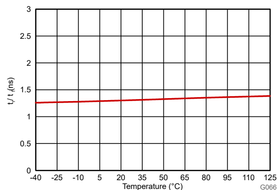
6-36. Output Rise and Fall Time vs Temperature
