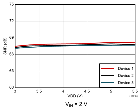
FIG 6-24. Signal-to-Noise Ratio vs Supply Voltage
