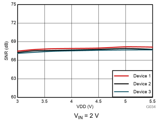
FIG 6-24. Signal-to-Noise Ratio vs Supply Voltage
