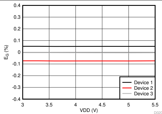
図 5-13. Gain Error vs Supply Voltage
