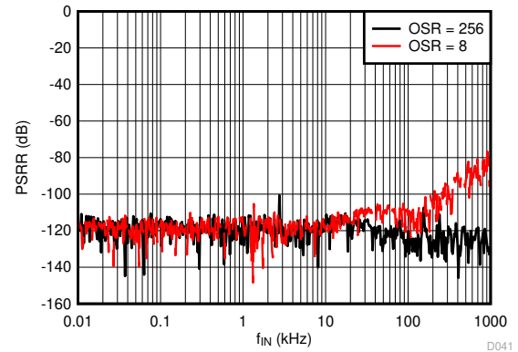
図 5-37. Power-Supply Rejection Ratio vs Ripple Frequency
