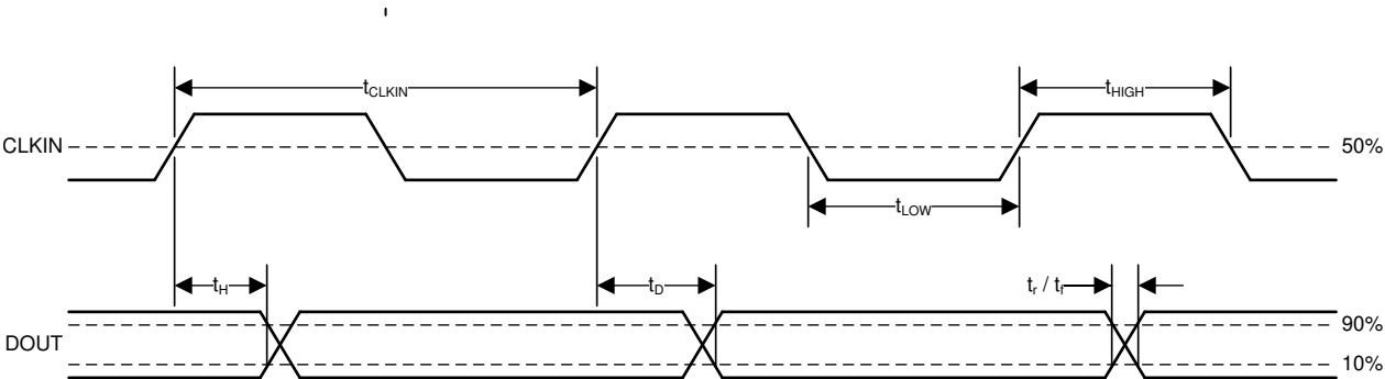
図 5-1. Digital Interface Timing
