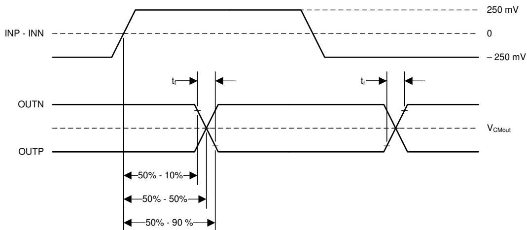
FIG 6-1. Rise, Fall, and Delay Time Waveforms
