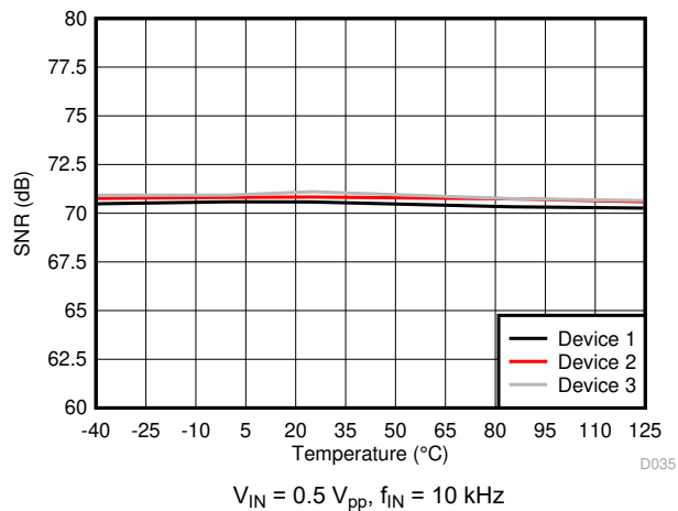
FIG 6-24. Signal-to-Noise Ratio vs Temperature
