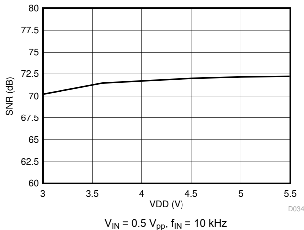
FIG 6-23. Signal-to-Noise Ratio vs Supply Voltage
