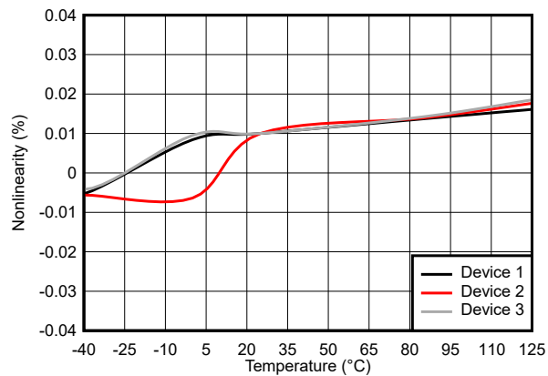
FIG 6-18. Nonlinearity vs Temperature
