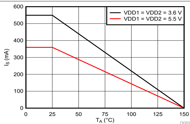
FIG 6-2. Thermal Derating Curve for Safety-Limiting Current per VDE
