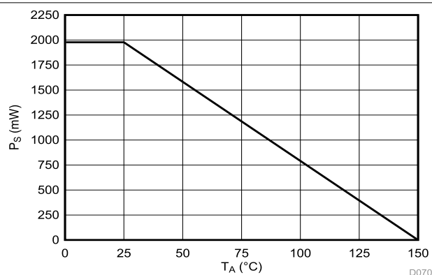
FIG 6-3. Thermal Derating Curve for Safety-Limiting Power per VDE
