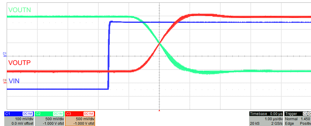
Figure 8-4. Step Response of the AMC1400
