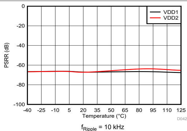
FIG 6-31. Power-Supply Rejection Ratio vs Temperature
