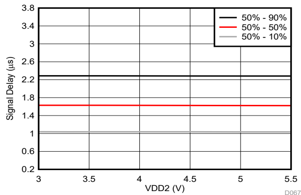
6-42. Input to Output Signal Delay vs Supply Voltage
