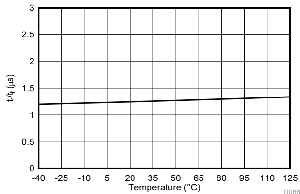
6-41. Output Rise and Fall Time vs Temperature
