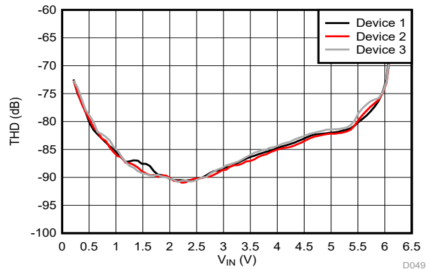
FIG 6-18. Total Harmonic Distortion vs Input Voltage
