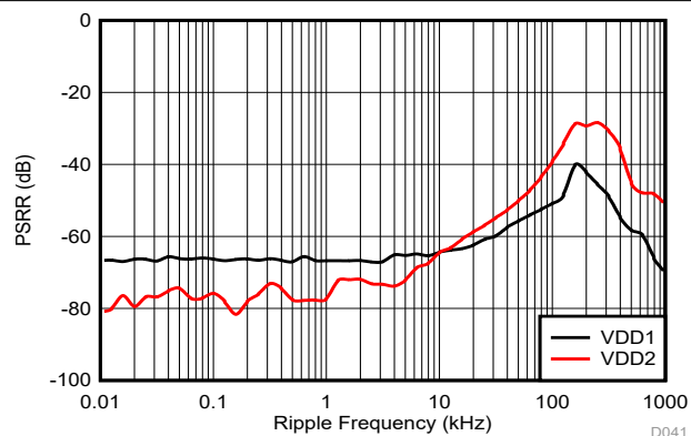
FIG 6-30. Power-Supply Rejection Ratio vs Ripple Frequency
