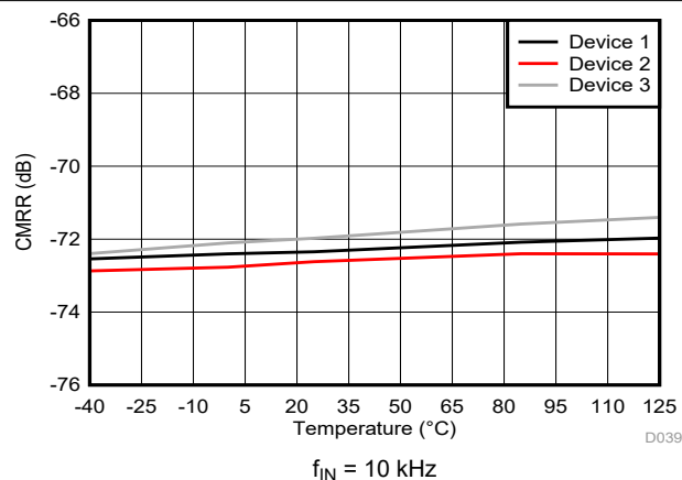
FIG 6-29. Common-Mode Rejection Ratio vs Temperature
