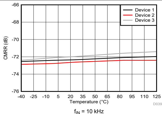
FIG 6-30. Common-Mode Rejection Ratio vs Temperature
