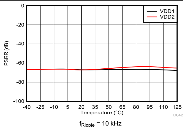
FIG 6-32. Power-Supply Rejection Ratio vs Temperature
