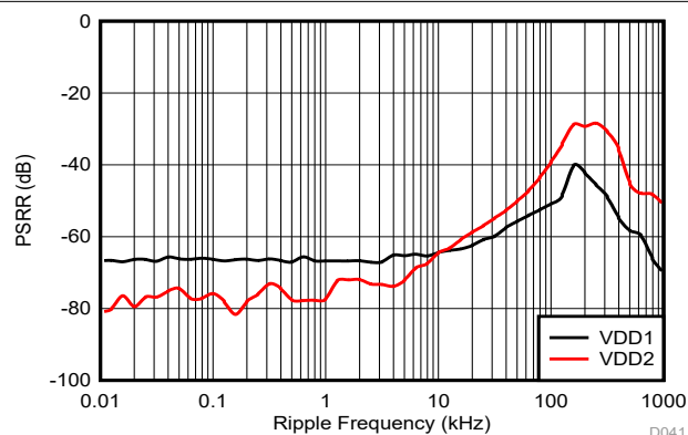
FIG 6-31. Power-Supply Rejection Ratio vs Ripple Frequency
