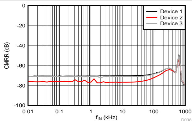
FIG 6-29. Common-Mode Rejection Ratio vs Input Frequency
