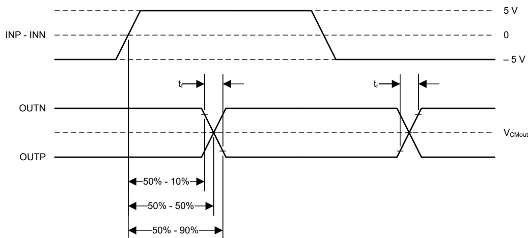
FIG 6-1. Rise, Fall, and Delay Time Definition
