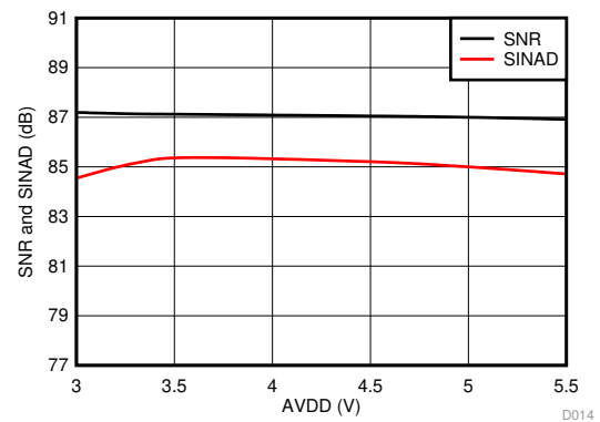
FIG 19. Signal-to-Noise Ratio and Signal-to-Noise + Distortion vs High-Side Supply Voltage
