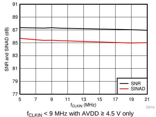
FIG 21. Signal-to-Noise Ratio and Signal-to-Noise + Distortion vs Clock Frequency
