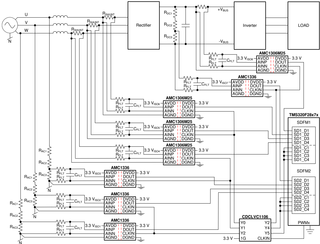
51. Input Phase Voltage Sensing Application with AMC1336
