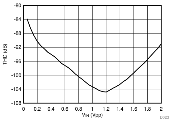
FIG 28. Total Harmonic Distortion vs Input Signal Amplitude
