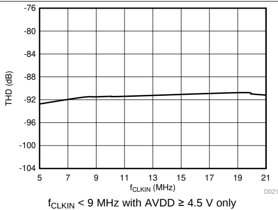
FIG 26. Total Harmonic Distortion vs Clock Frequency
