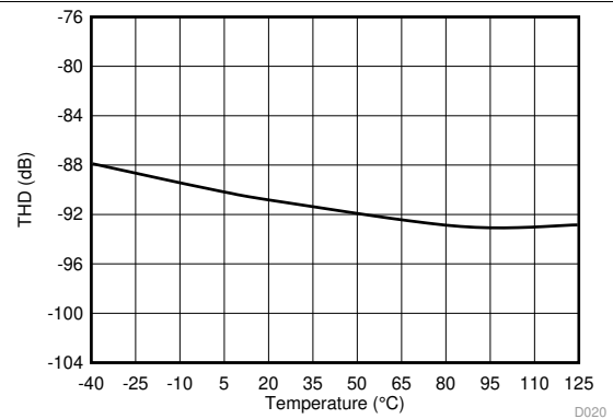
FIG 25. Total Harmonic Distortion vs Temperature
