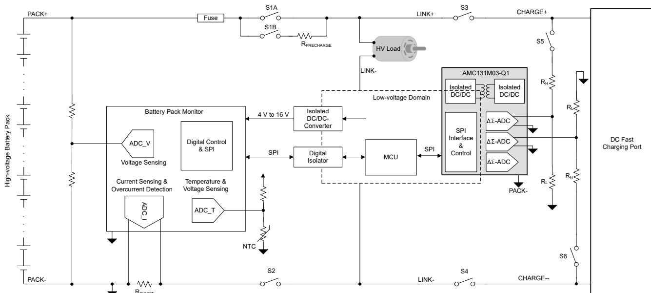
図 9-4. AMC131M03-Q1 in a Typical Battery Management System Application
