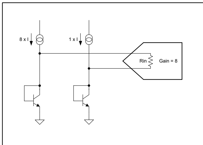
図 8-15. Internal Temperature Sensor Block Diagram
