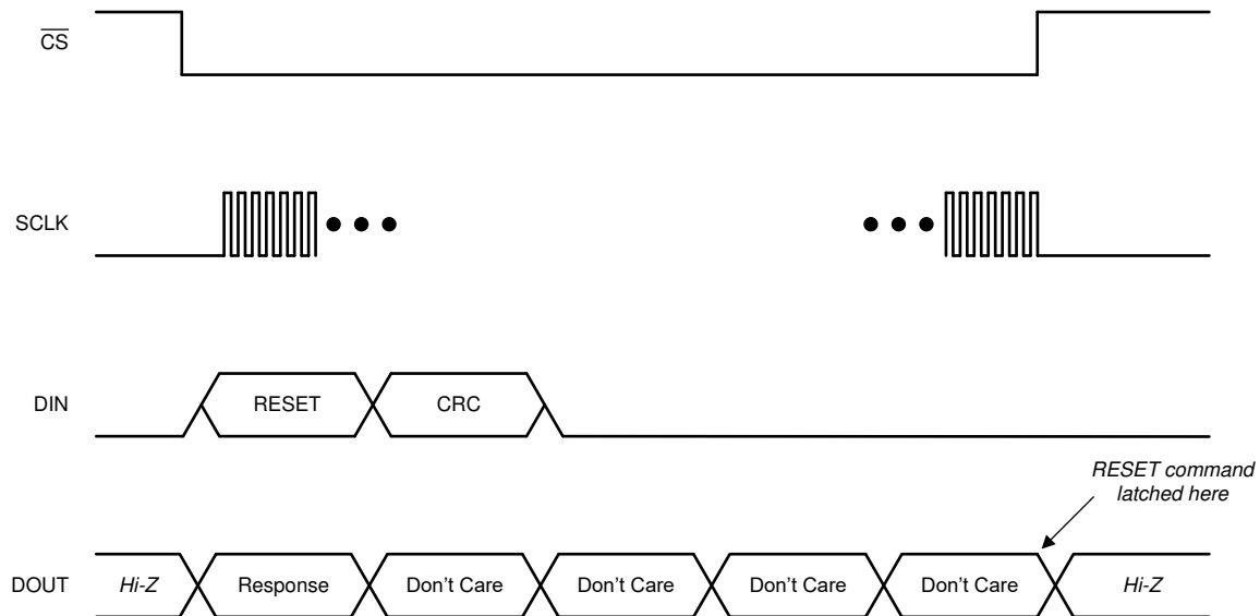
8-26. RESET Command Frame
