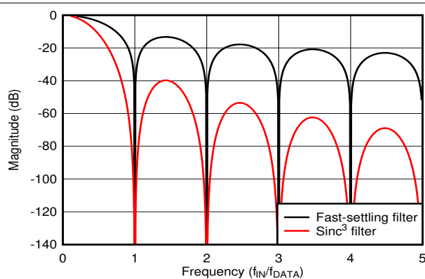
図 8-7. Fast-Settling and Sinc 3 Digital Filter Response
