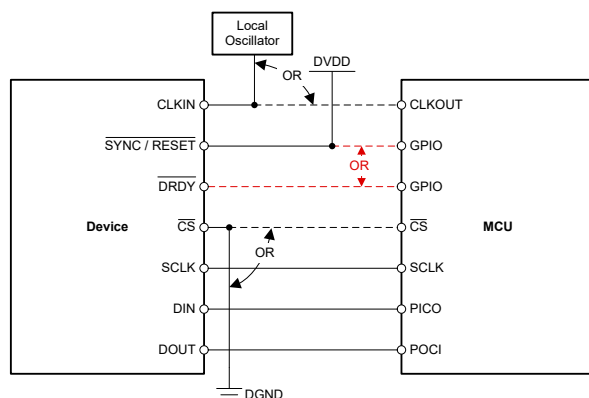
図 9-2. Minimum Connections Required to Operate the AMC131M03
