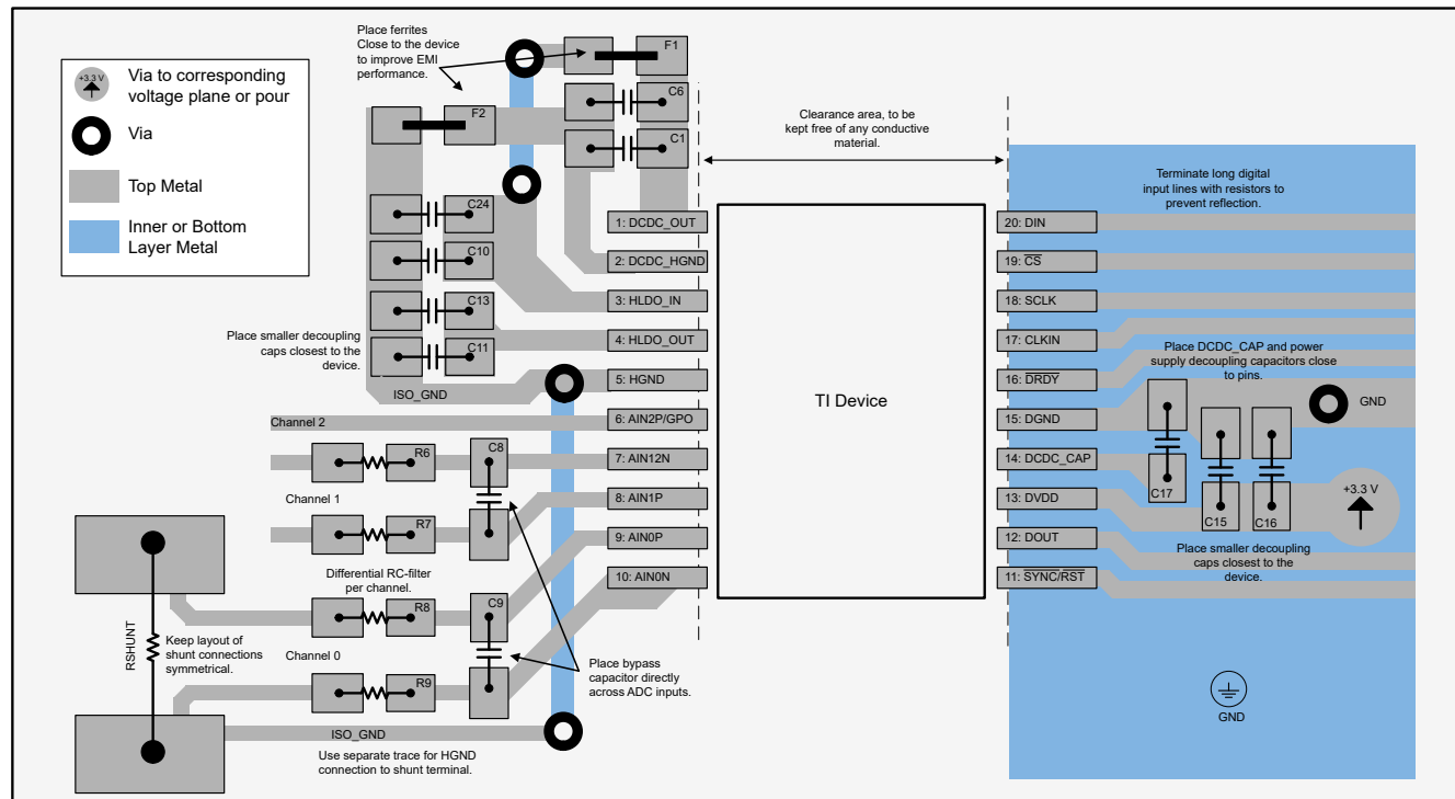
Figure 9-9. Layout Example
