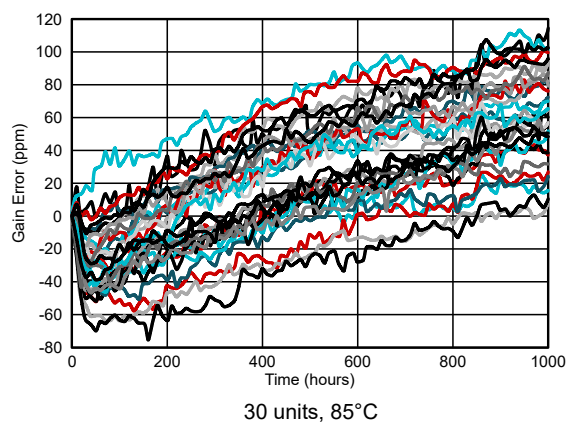
Figure 6-11. Gain Error vs Time
