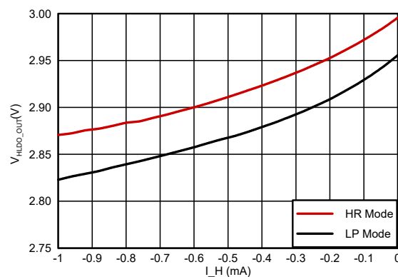
6-23. HLDO Output Voltage vs Load Current
