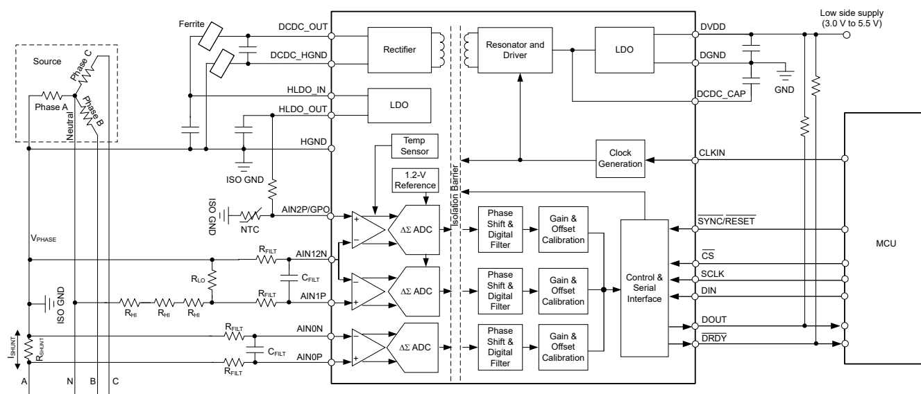
9-5. Current and Voltage Sensing With the AMC131M03
