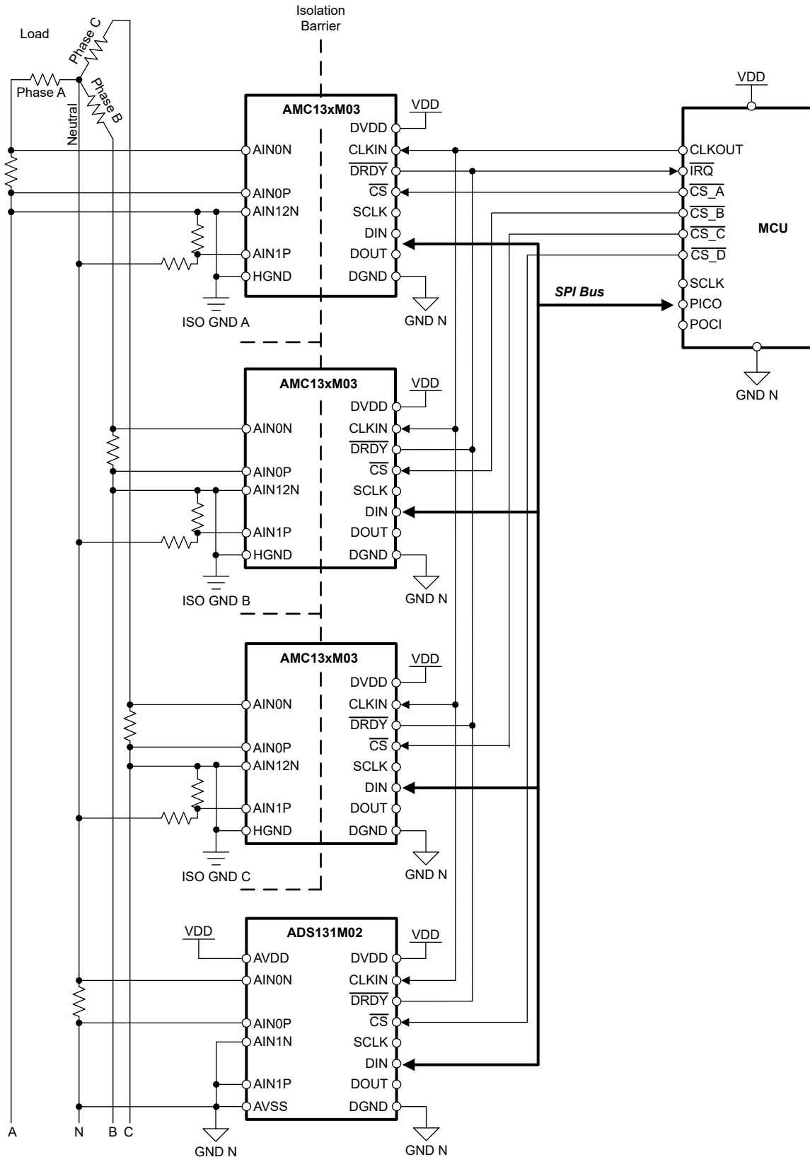
図 9-4. 3-Phase Metrology Design Front-End Using the AMC131M03
