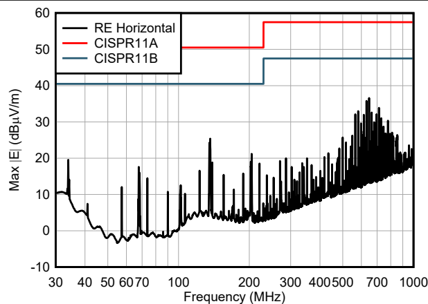
☒ 9-6. AMC131M02 Horizontal Radiated Emission CISPR11 Measurement
