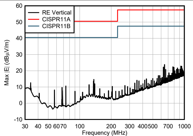
☒ 9-7. AMC131M02 Vertical Radiated Emission CISPR11 Measurement
