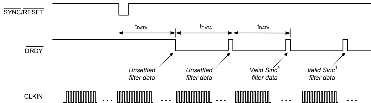
✎ 8-19. Synchronization Timing for OSR = 1024
