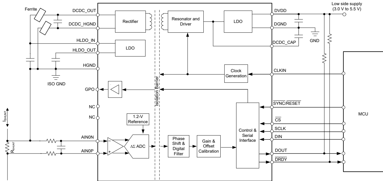
図 9-5. Current Sensing With the AMC131M01
