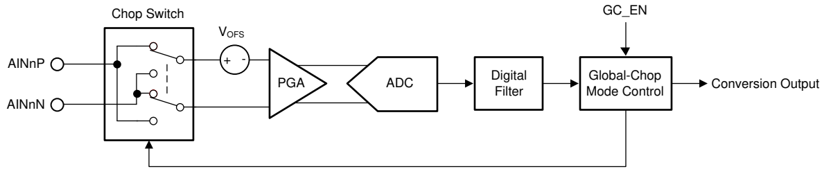
図 8-17. Global-Chop Mode Implementation
