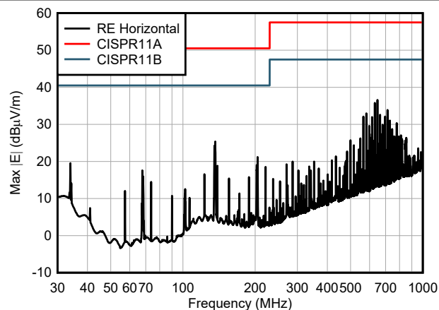
図 9-6. AMC131M01 Horizontal Radiated Emission CISPR11 Measurement
