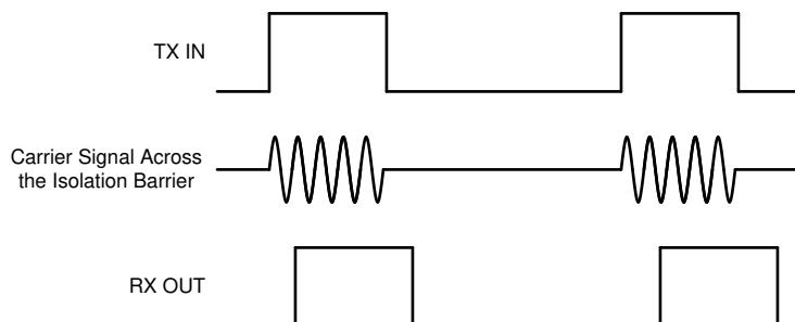
8-2. OOK-Based Modulation Scheme
