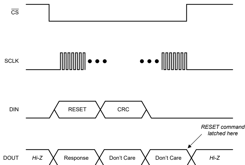
8-21. RESET Command Frame
