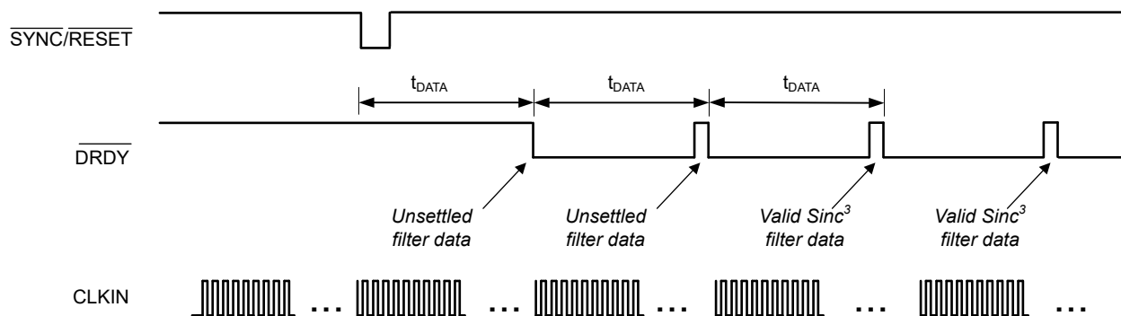
✕ 8-16. Synchronization Timing for OSR = 1024
