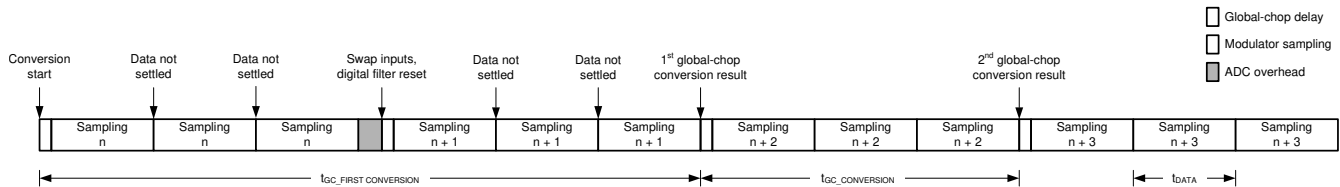
図 8-18. Conversion Timing With Global-Chop Mode Enabled
