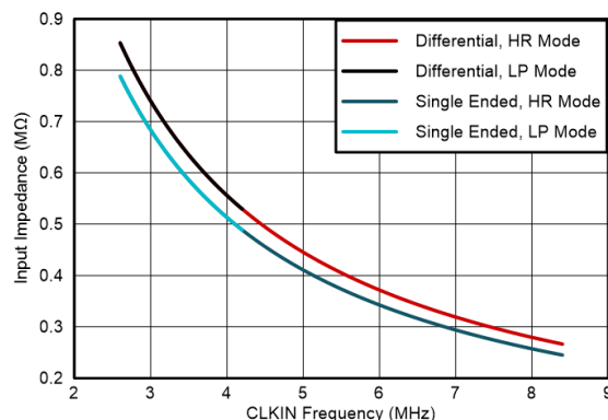
図 6-5. Input Impedance vs CLKIN Frequency
