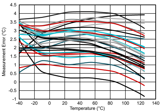
图 6-16. Internal Temperature Sensor Accuracy vs Temperature (Without Calibration)
