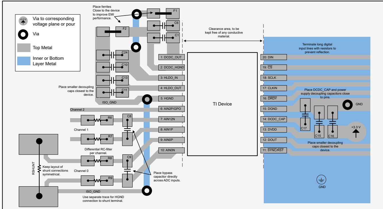
Figure 9-9. Layout Example
