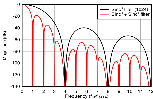
図 8-9. Digital Filter Response for OSR = 4096 as a Combination of Sinc 3 + Sinc 1
