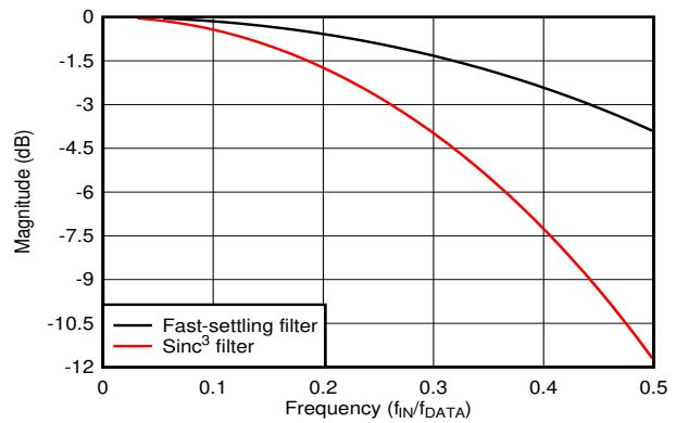
図 8-8. Fast-Settling and Sinc 3 Digital Filter Response, Pass-Band Detail
