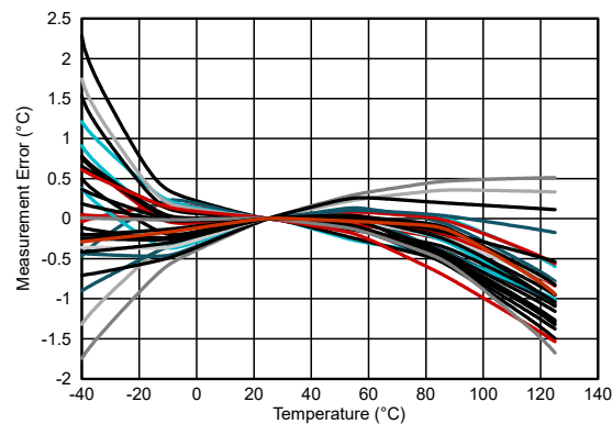
图 6-17. Internal Temperature Sensor Accuracy vs Temperature (With Calibration)
