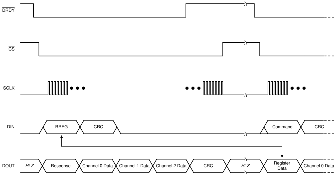
図 8-27. Reading a Single Register
