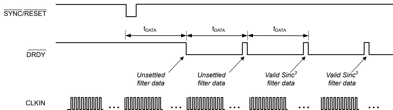
✎ 8-21. Synchronization Timing for OSR = 1024
