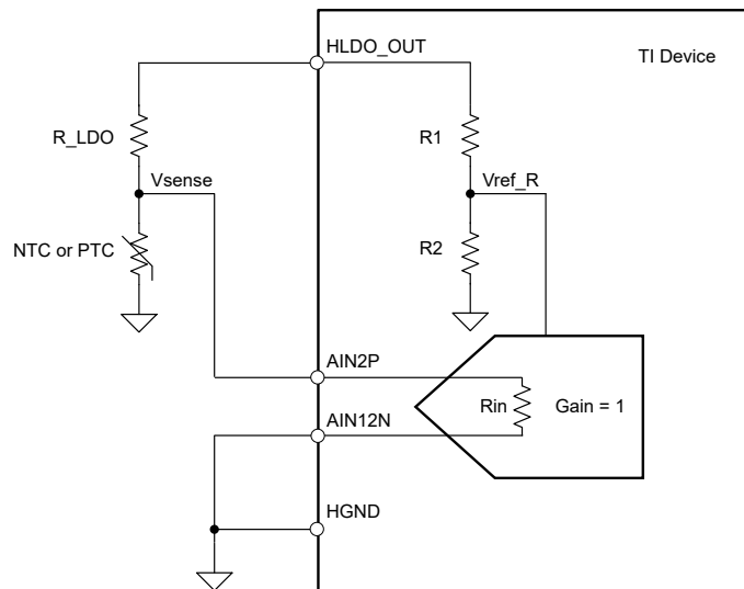
図 8-16. External Temperature Sensor Measurement Block Diagram
