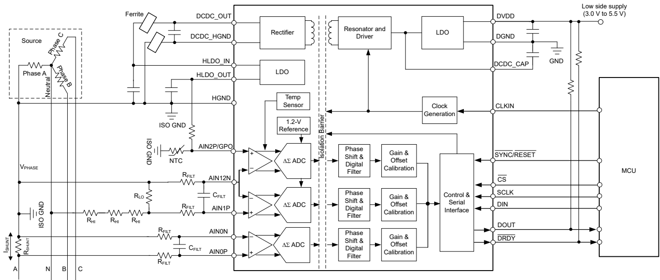
図 9-5. Current and Voltage Sensing With the AMC130M03
