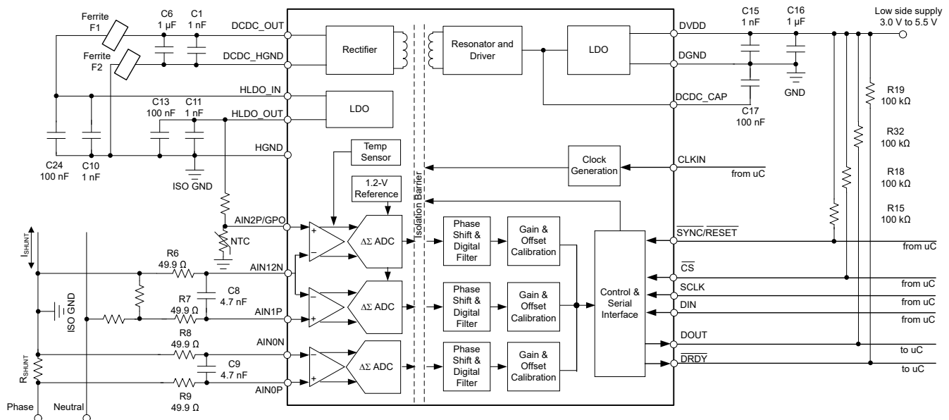
図 9-8. Power Supply Decoupling the AMC130M03
