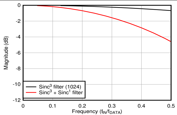
図 8-10. Sinc 3 + Sinc 1 Digital Filter Response at OSR = 4096, Pass-Band Detail
