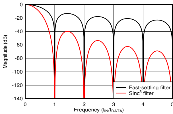
図 8-7. Fast-Settling and Sinc 3 Digital Filter Response
