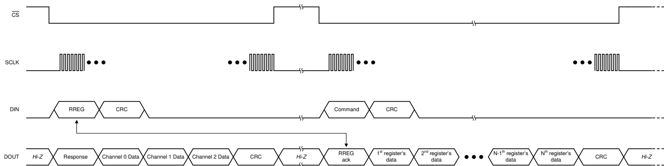
図 8-28. Reading Multiple Registers
