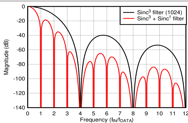
図 8-9. Digital Filter Response for OSR = 4096 as a Combination of Sinc 3 + Sinc 1
