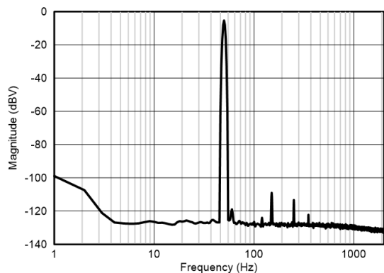
図 6-14. Frequency Spectrum With 50-Hz Input Signal
