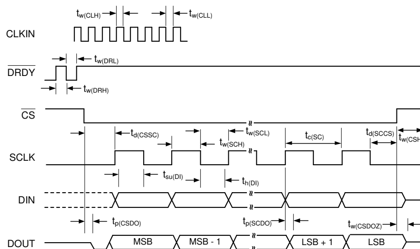
図 6-1. SPI Timing Diagram
