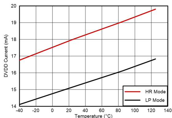
図 6-17. DVDD Current vs Temperature
