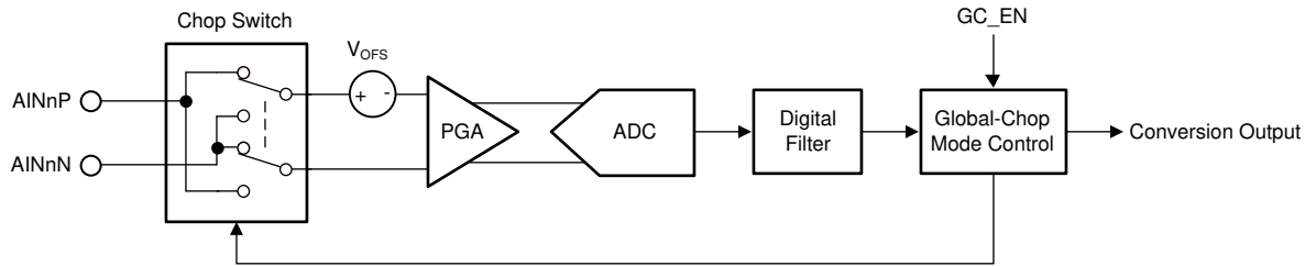
図 8-20. Global-Chop Mode Implementation
