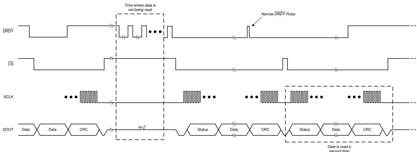
図 8-30. Collecting Data After a Pause by Reading Data Twice
