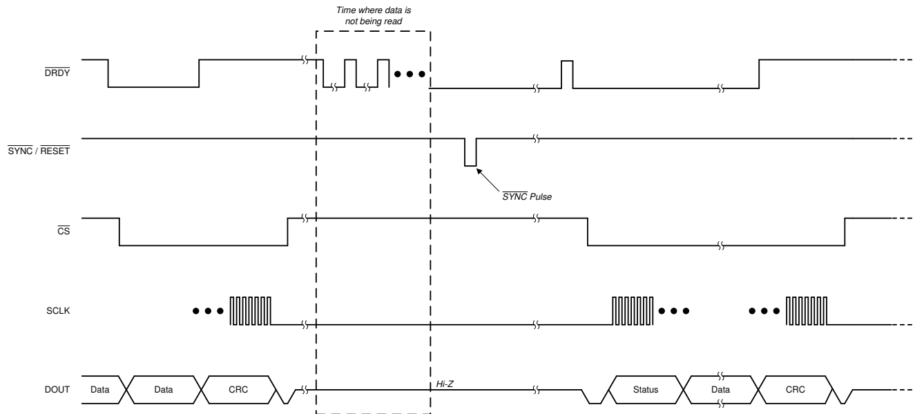
図 8-29. Collecting Data After a Pause Using the SYNC/RESET Pin
