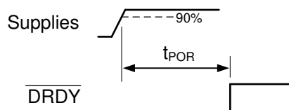
図 6-3. Power-On-Reset Timing
