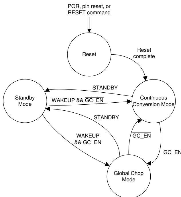
図 8-15. State Diagram Depicting Device Functional Modes
