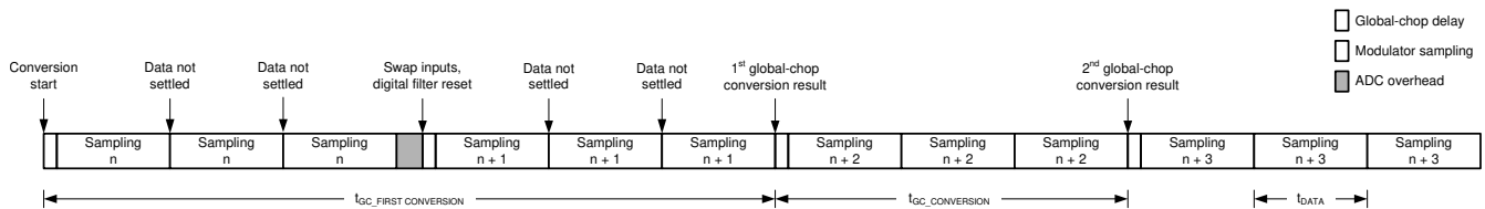
図 8-21. Conversion Timing With Global-Chop Mode Enabled
