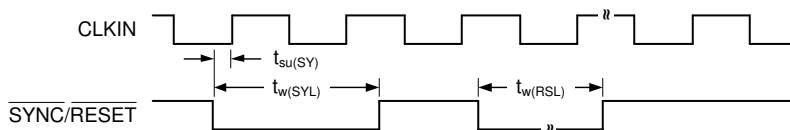
図 6-2. SYNC/RESET Timing Requirements
