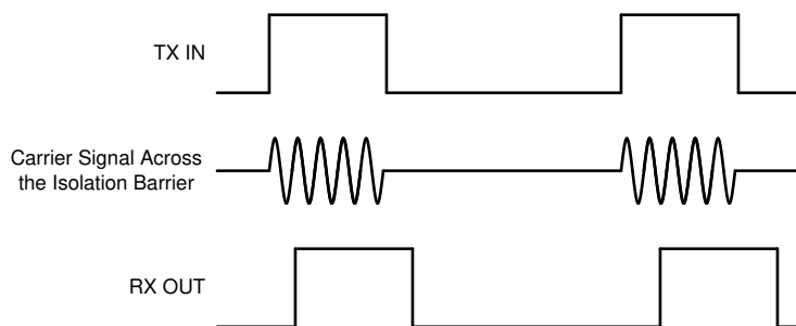
図 8-2. OOK-Based Modulation Scheme
