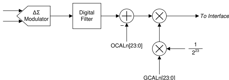
図 8-14. Calibration Block Diagram
