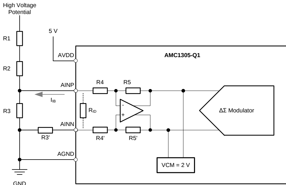
Figure 56. Using AMC1305-Q1 for Isolated Voltage Sensing
