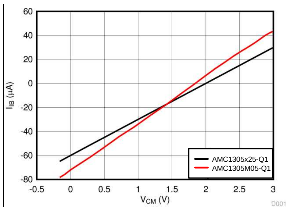
Figure 6. Input Current vs Input Common-Mode Voltage
