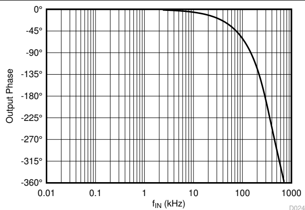
FIG 6-17. Output Phase vs Input Frequency
