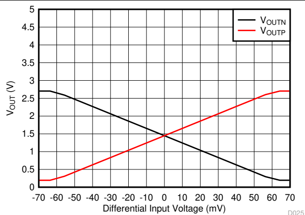
FIG 6-18. Output Voltage vs Input Voltage
