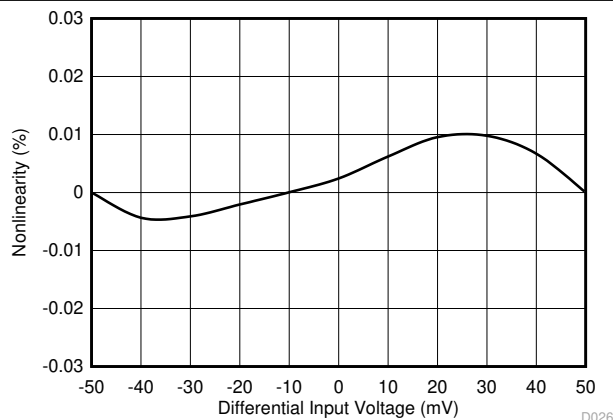
FIG 6-19. Nonlinearity vs Input Voltage
