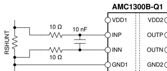
図 8-2. Differential Input Filter
