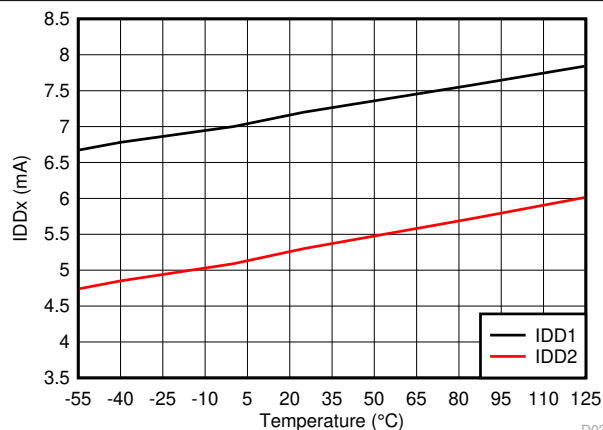
Figure 7-36. Supply Current vs Temperature
