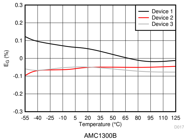
7-17. Gain Error vs Temperature
