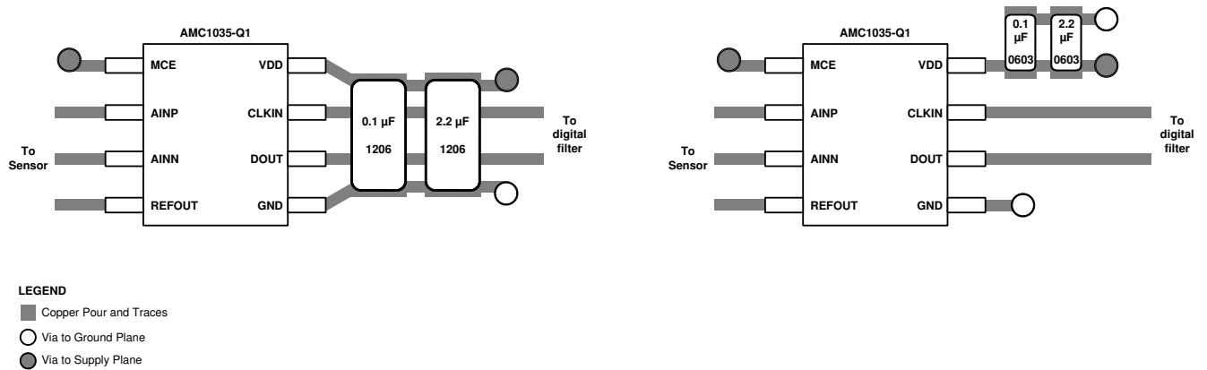
Figure 50. Recommended Layout of the AMC1035-Q1
