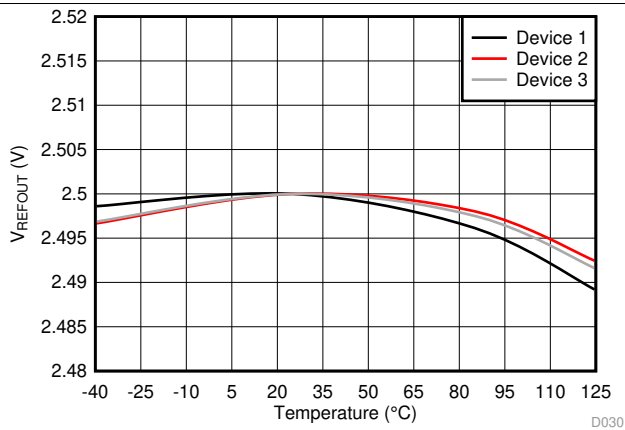
FIG 33. Reference Output Voltage vs Temperature
