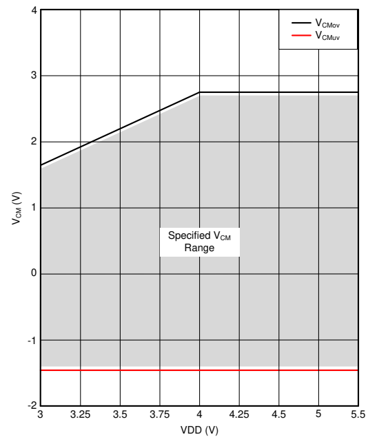
Figure 39. Common-Mode Input Voltage Range With a Zero Differential Input Signal
