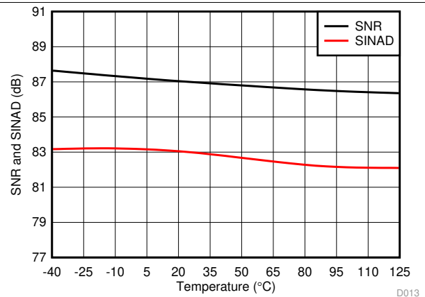
FIG 16. Signal-to-Noise Ratio and Signal-to-Noise + Distortion vs Temperature
