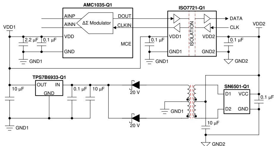
FIG 49. Galvanic Isolation of the AMC1035-Q1
