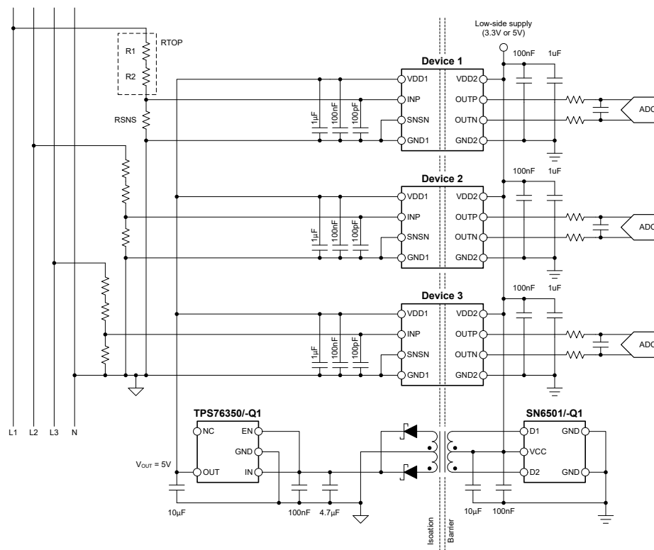
Figure 8-1. Using the AMC0x30D in a Typical Application
