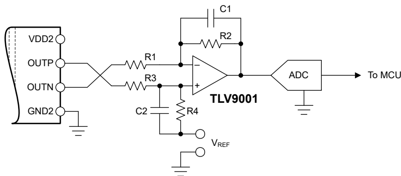
Figure 8-3. Connecting the AMC0x30D Output to a Single-Ended Input ADC
