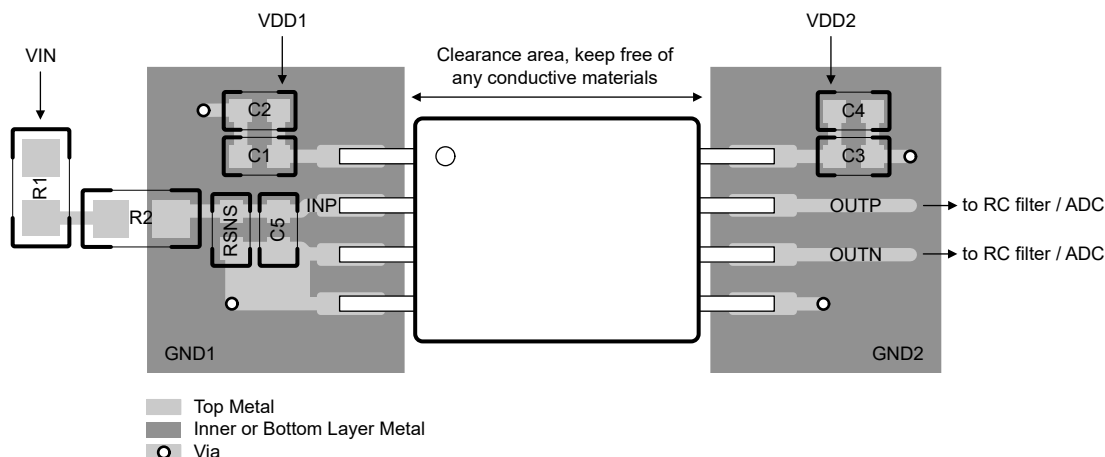
Figure 8-6. Recommended Layout of the AMC0x30D
