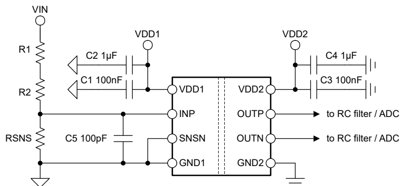
Figure 8-5. Decoupling of the AMC0x30D
