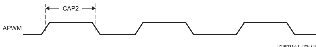
図 6-30. ECAP Switching Characteristics
