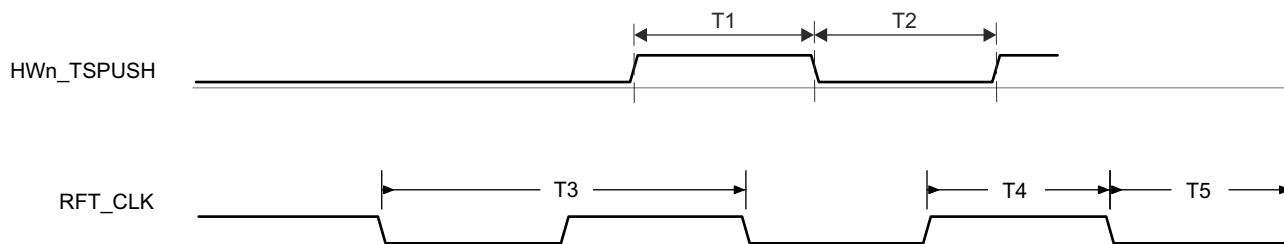
図 6-76. CPTS Timing Requirements
